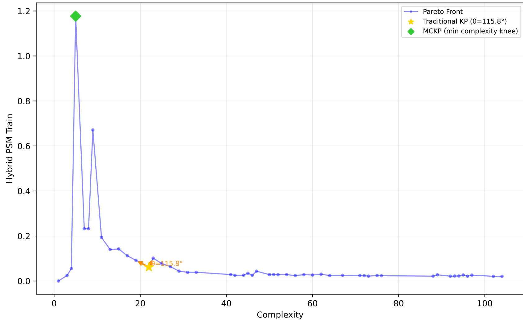
227_cpu_small - Run 2 - SVP - Hybrid PSM Train \lambda_1=0.00, \bar{\lambda}_2=1.00, \lambda_3=0.00 | Difficulty: 1.00 | Method: hmr
