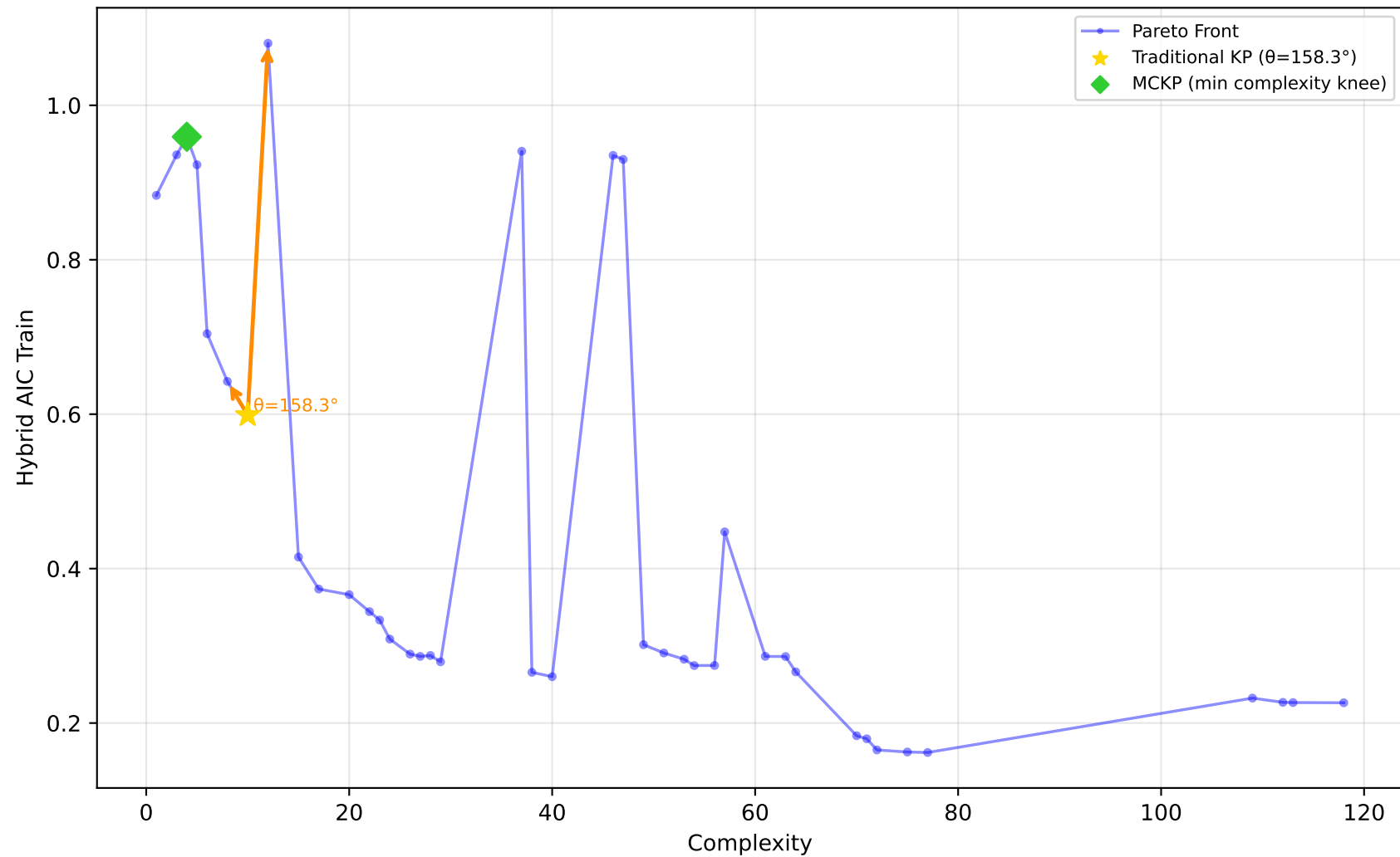
227_cpu_small - Run 30 - MVP - Hybrid AIC Train \lambda_1=0.80, \bar{\lambda}_2=0.20, \lambda_3=0.00 | Difficulty: 1.00 | Method: hmr
