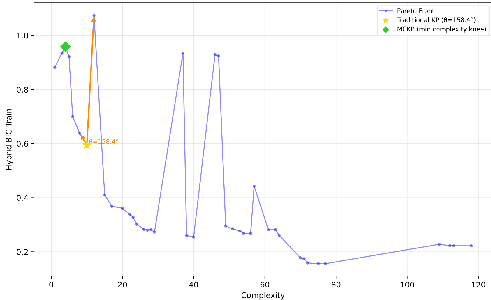
227_cpu_small - Run 30 - MVP - Hybrid BIC Train \lambda_1=0.80, \bar{\lambda}_2=0.20, \lambda_3=0.00 | Difficulty: 1.00 | Method: hmr
