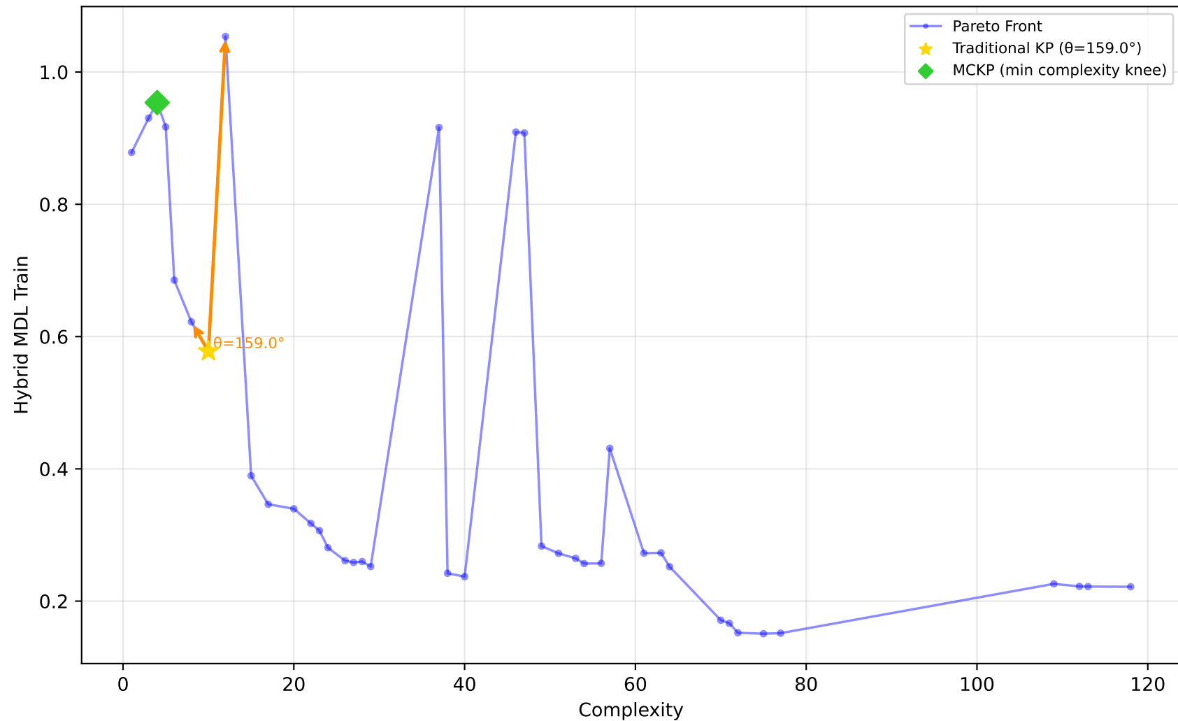
227_cpu_small - Run 30 - MVP - Hybrid MDL Train \lambda_1=0.80, \lambda_2=0.20, \lambda_3=0.00 | Difficulty: 1.00 | Method: hmr
