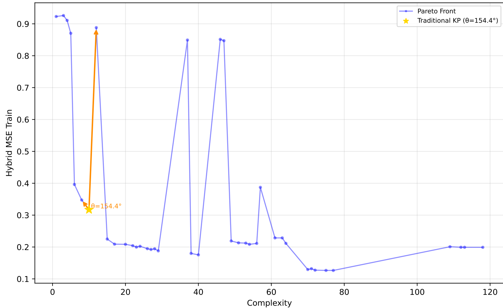
227_cpu_small - Run 30 - MVP - Hybrid MSE Train \lambda_1=0.80, \lambda_2=0.20, \lambda_3=0.00 | Difficulty: 1.00 | Method: hmr
