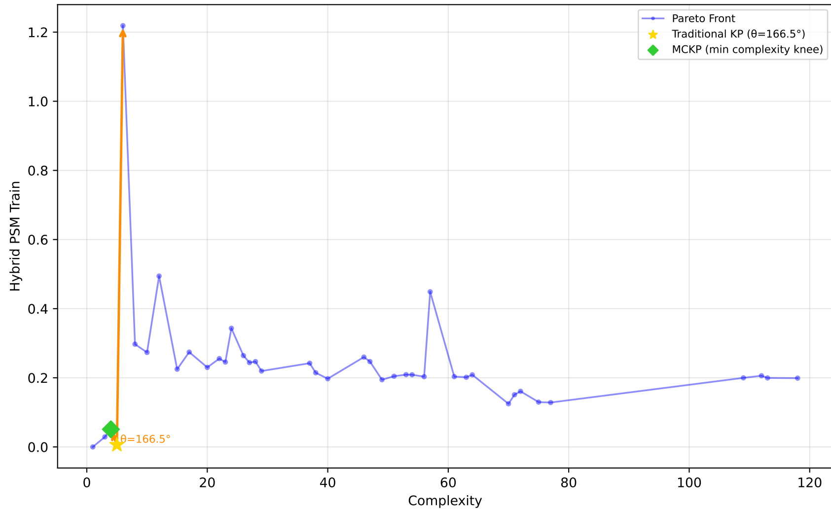
227_cpu_small - Run 30 - MVP - Hybrid PSM Train \lambda_1=0.00, \lambda_2=0.90, \lambda_3=0.10 | Difficulty: 1.00 | Method: hmr
