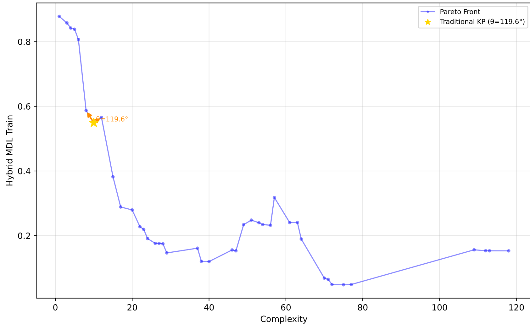
227_cpu_small - Run 30 - SVP - Hybrid MDL Train \lambda_1=0.00, \lambda_2=0.80, \lambda_3=0.30 | Difficulty: 1.00 | Method: hmr
