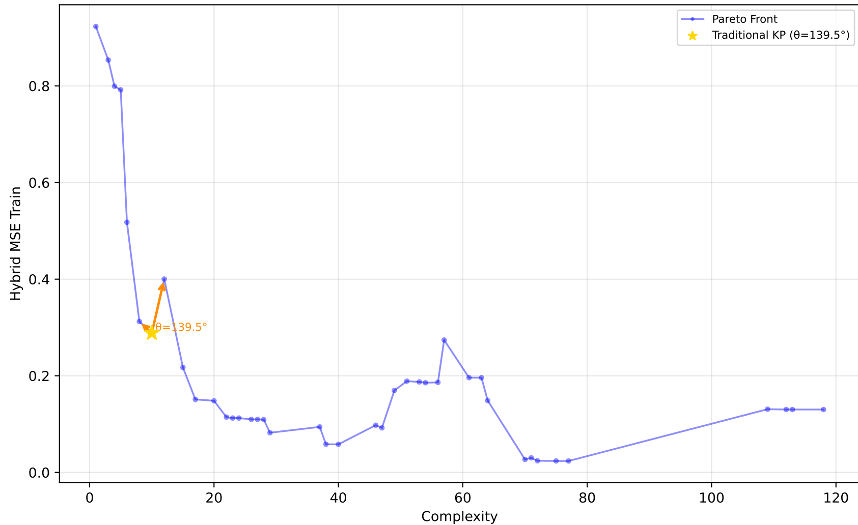
227_cpu_small - Run 30 - SVP - Hybrid MSE Train \lambda_1=0.00, \lambda_2=0.80, \lambda_3=0.30 | Difficulty: 1.00 | Method: hmr
