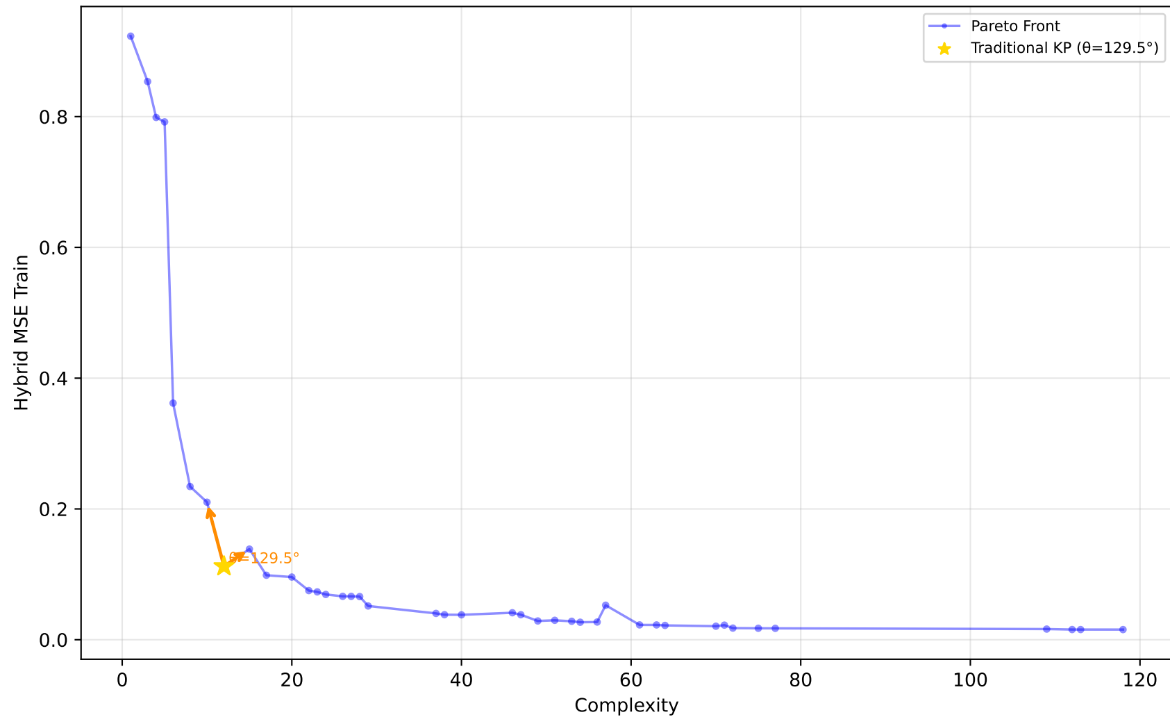
227_cpu_small - Run 30 - SVP - Hybrid MSE Train \lambda_1=0.00, \lambda_2=1.00, \lambda_3=0.00 | Difficulty: 1.00 | Method: hmr
