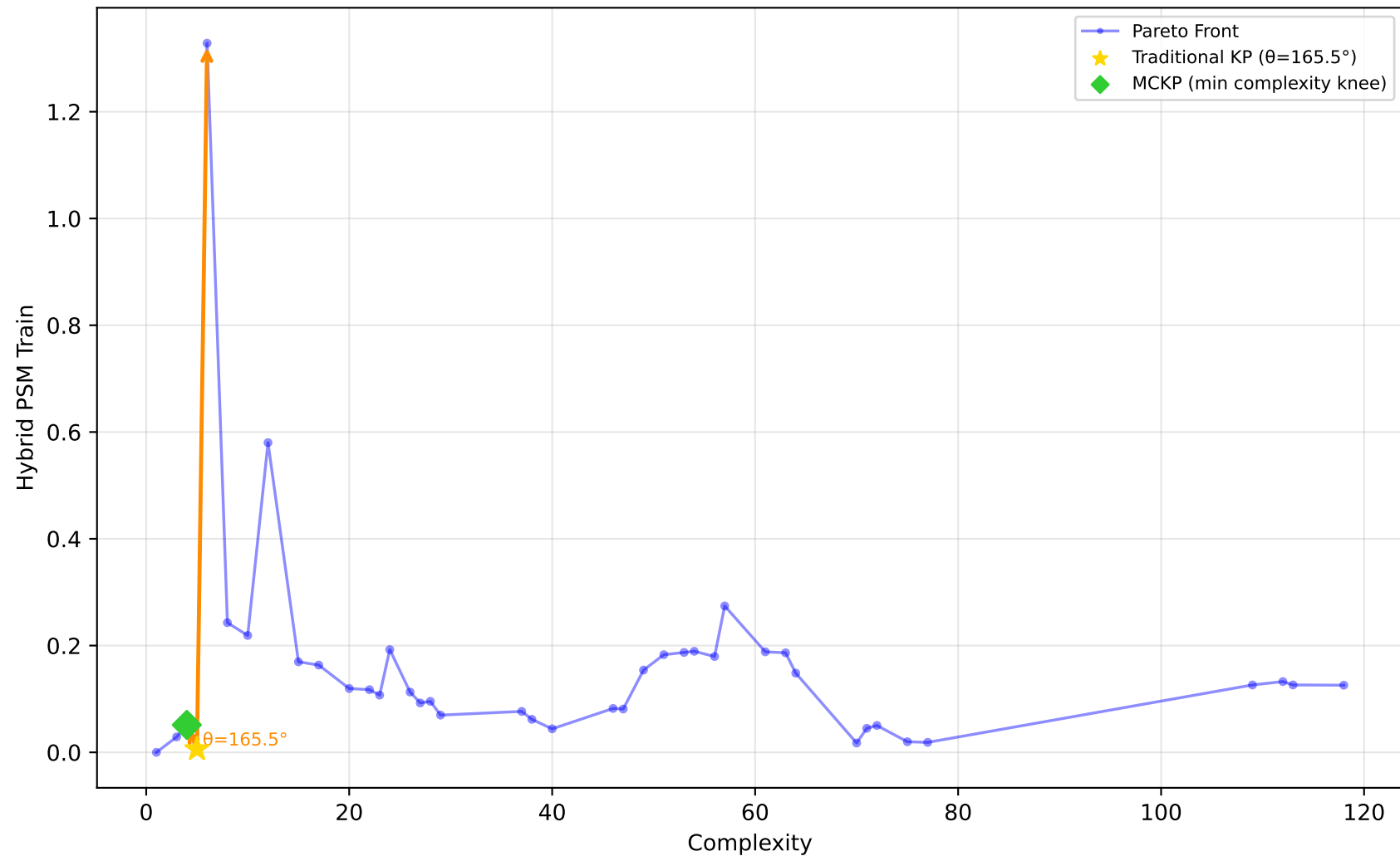
227_cpu_small - Run 30 - SVP - Hybrid PSM Train \lambda_1=0.00, \lambda_2=0.80, \lambda_3=0.30 | Difficulty: 1.00 | Method: hmr
