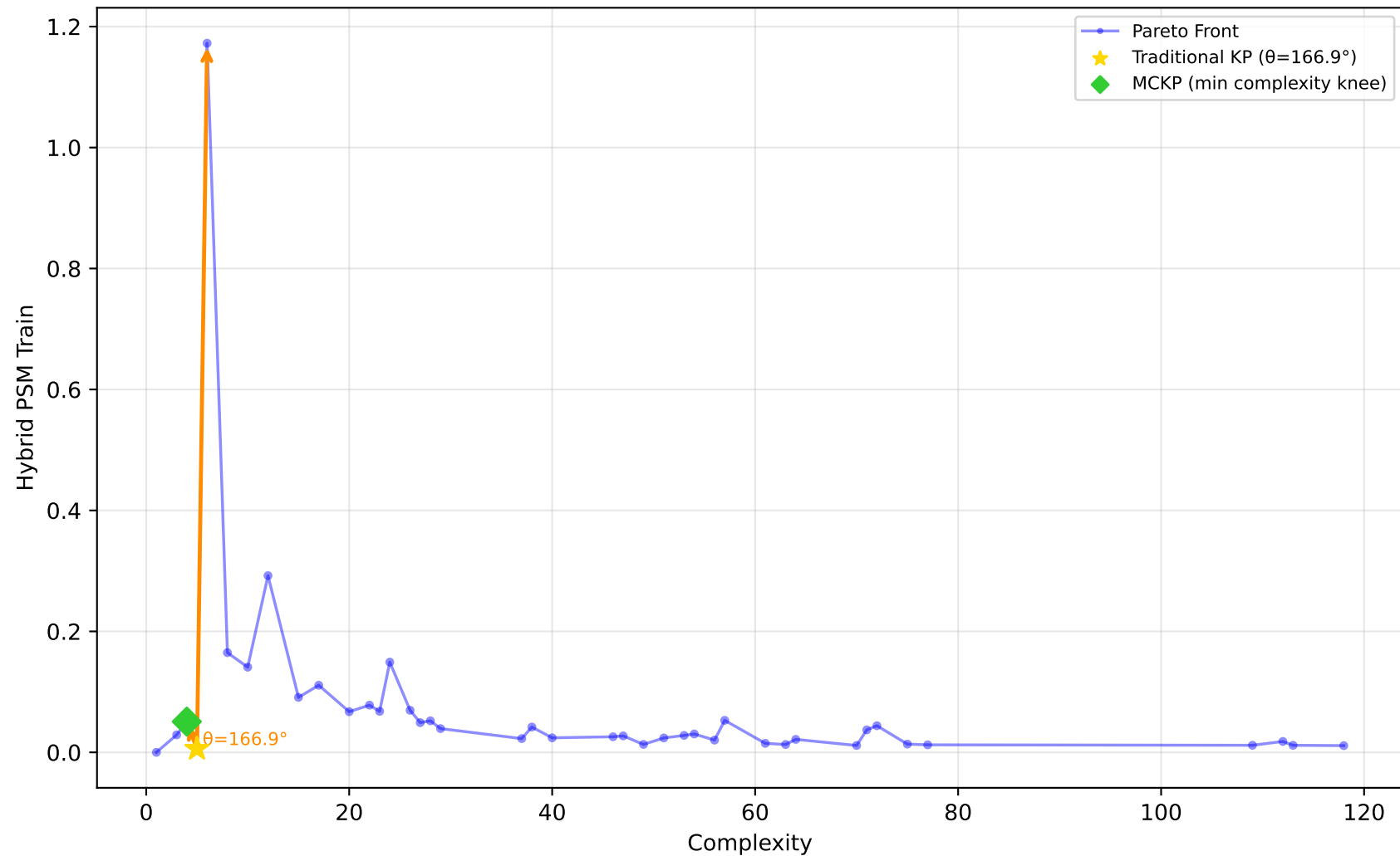
227_cpu_small - Run 30 - SVP - Hybrid PSM Train \lambda_1=0.00, \lambda_2=1.00, \lambda_3=0.00 | Difficulty: 1.00 | Method: hmr
