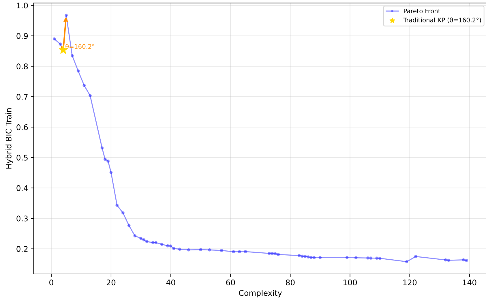
227_cpu_small - Run 3 - MVP - Hybrid BIC Train \lambda_1=0.00, \bar{\lambda}_2=0.90, \lambda_3=0.10 | Difficulty: 1.00 | Method: hmr
