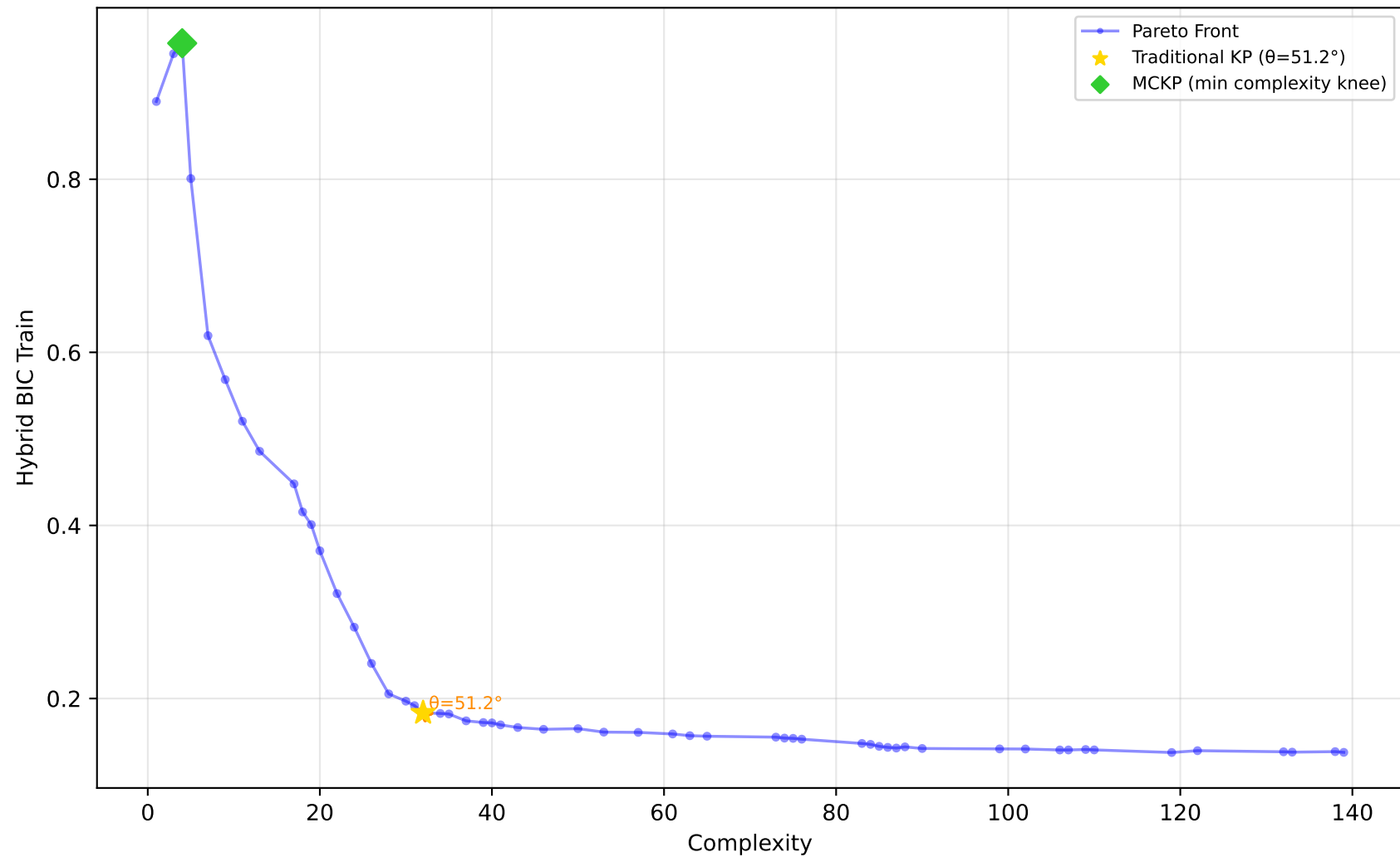
227_cpu_small - Run 3 - MVP - Hybrid BIC Train \lambda_1=0.80, \bar{\lambda}_2=0.20, \lambda_3=0.00 | Difficulty: 1.00 | Method: hmr
