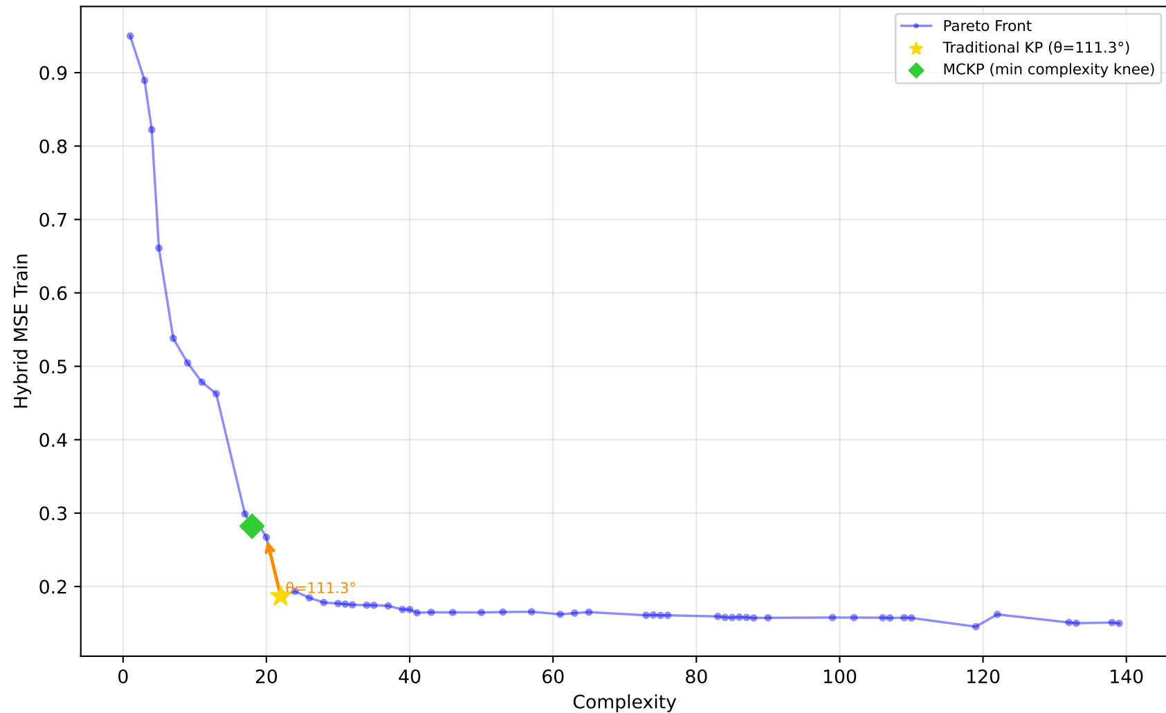
227_cpu_small - Run 3 - MVP - Hybrid MSE Train \lambda_1=0.00, \lambda_2=0.90, \lambda_3=0.10 | Difficulty: 1.00 | Method: hmr
