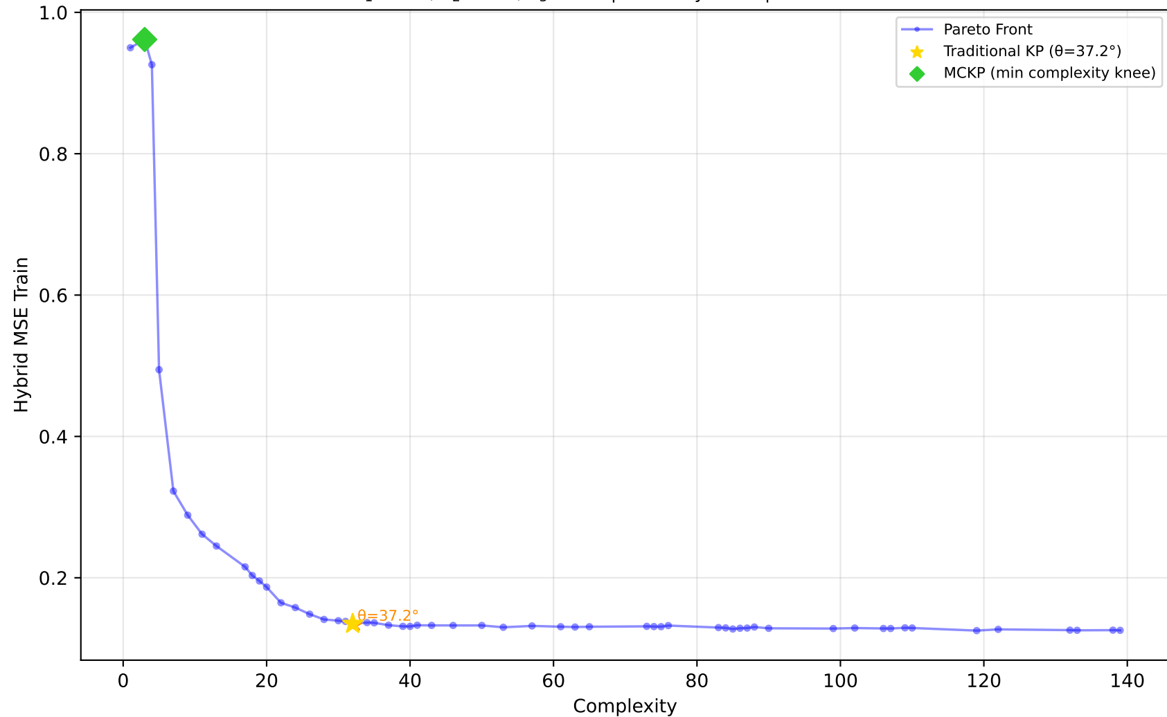
227_cpu_small - Run 3 - MVP - Hybrid MSE Train \lambda_1=0.80, \bar{\lambda}_2=0.20, \lambda_3=0.00 | Difficulty: 1.00 | Method: hmr
