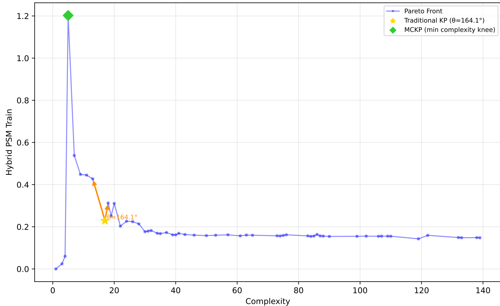
227_cpu_small - Run 3 - MVP - Hybrid PSM Train \lambda_1=0.00, \bar{\lambda}_2=0.90, \lambda_3=0.10 | Difficulty: 1.00 | Method: hmr
