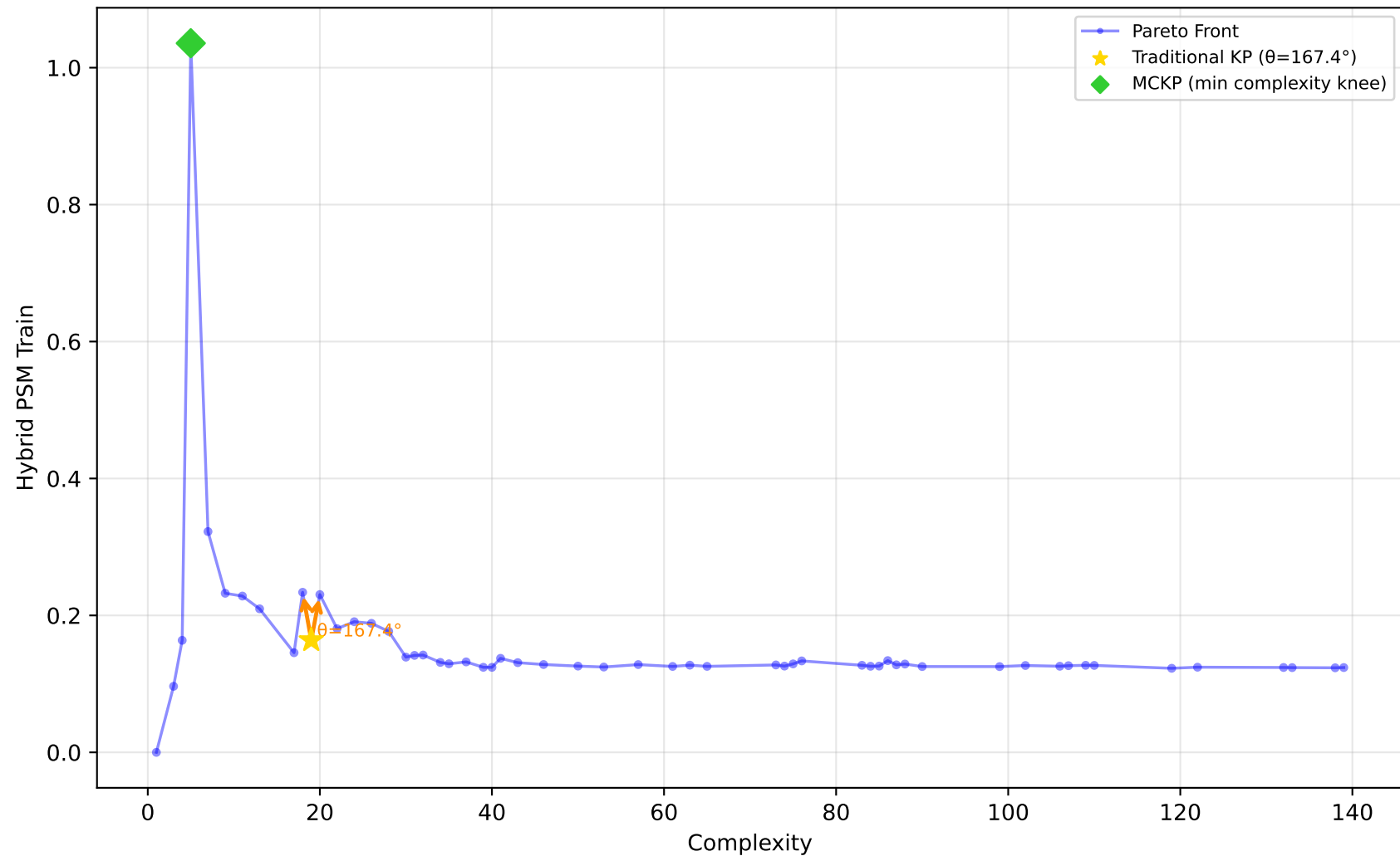
227_cpu_small - Run 3 - MVP - Hybrid PSM Train \lambda_1=0.80, \bar{\lambda}_2=0.20, \lambda_3=0.00 | Difficulty: 1.00 | Method: hmr
