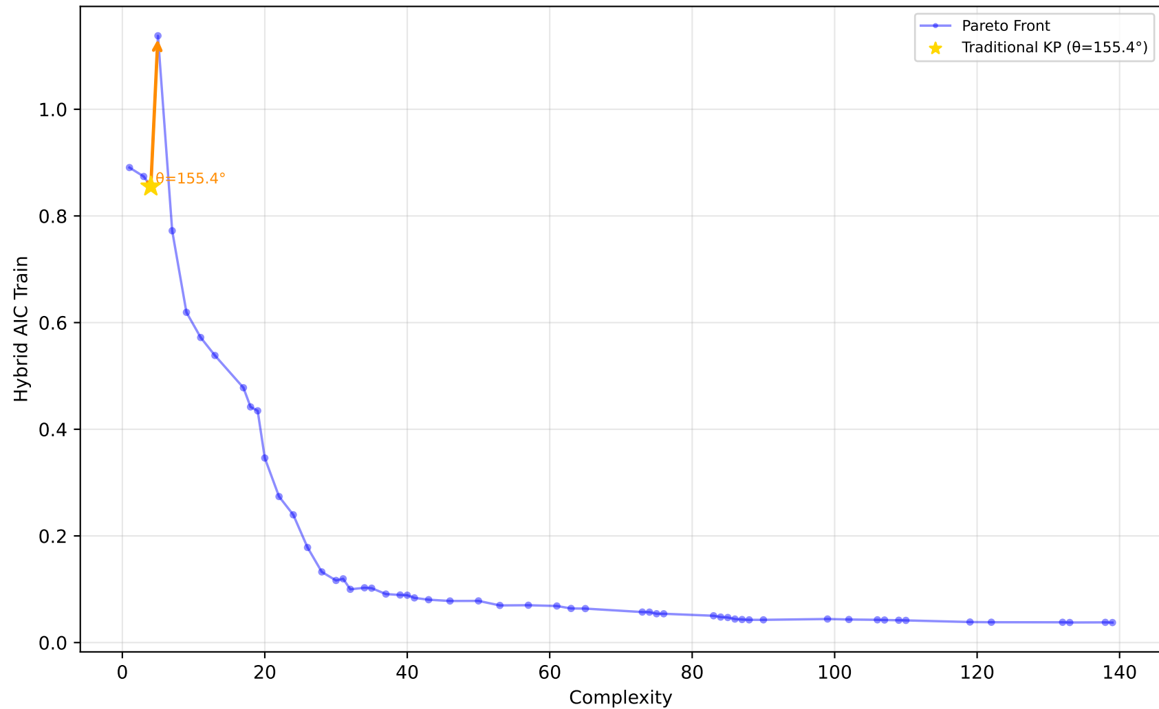
227_cpu_small - Run 3 - SVP - Hybrid AIC Train \lambda_1=0.00, \bar{\lambda}_2=0.80, \lambda_3=0.30 | Difficulty: 1.00 | Method: hmr
