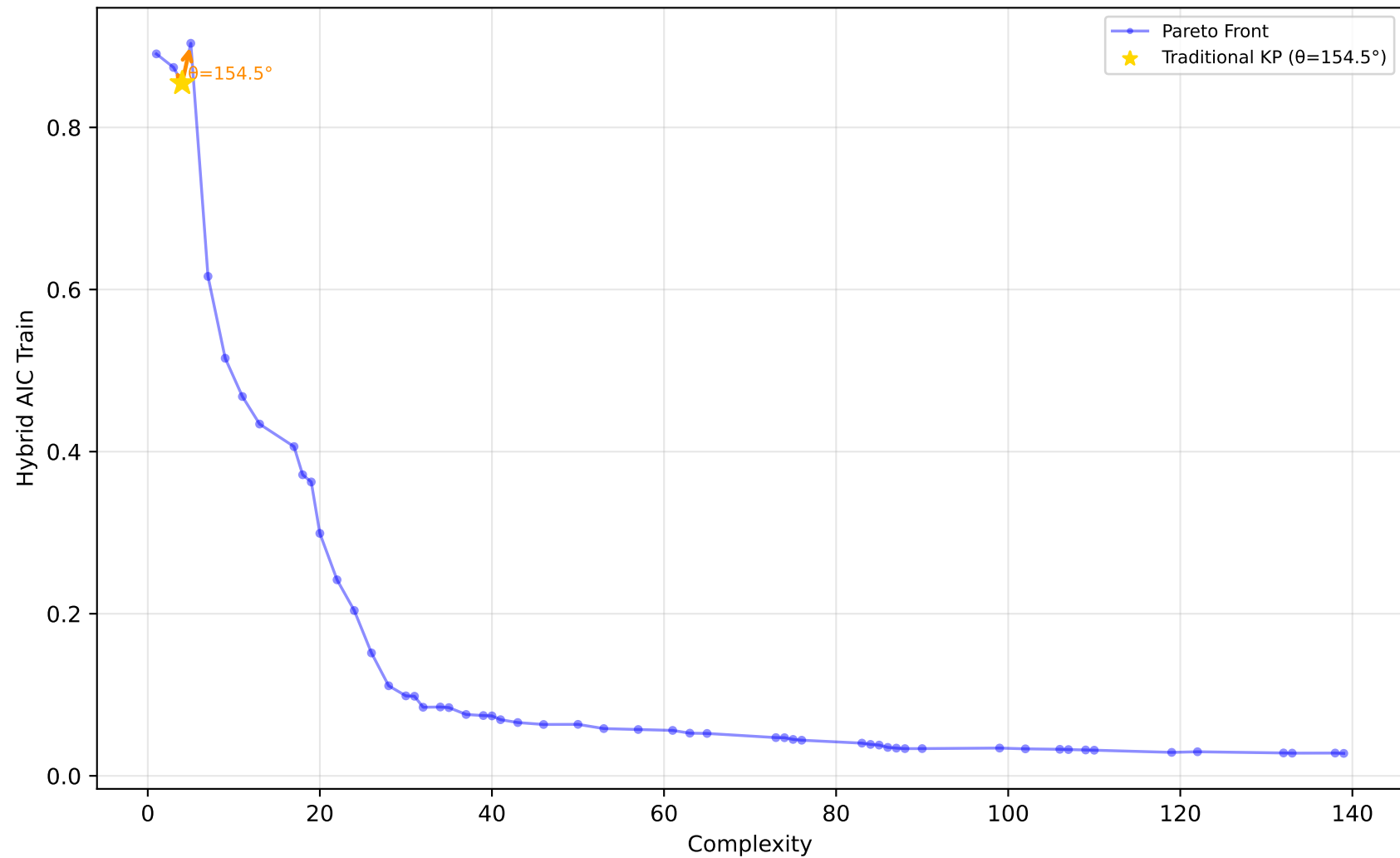
227_cpu_small - Run 3 - SVP - Hybrid AIC Train \lambda_1=0.00, \lambda_2=1.00, \lambda_3=0.00 | Difficulty: 1.00 | Method: hmr
