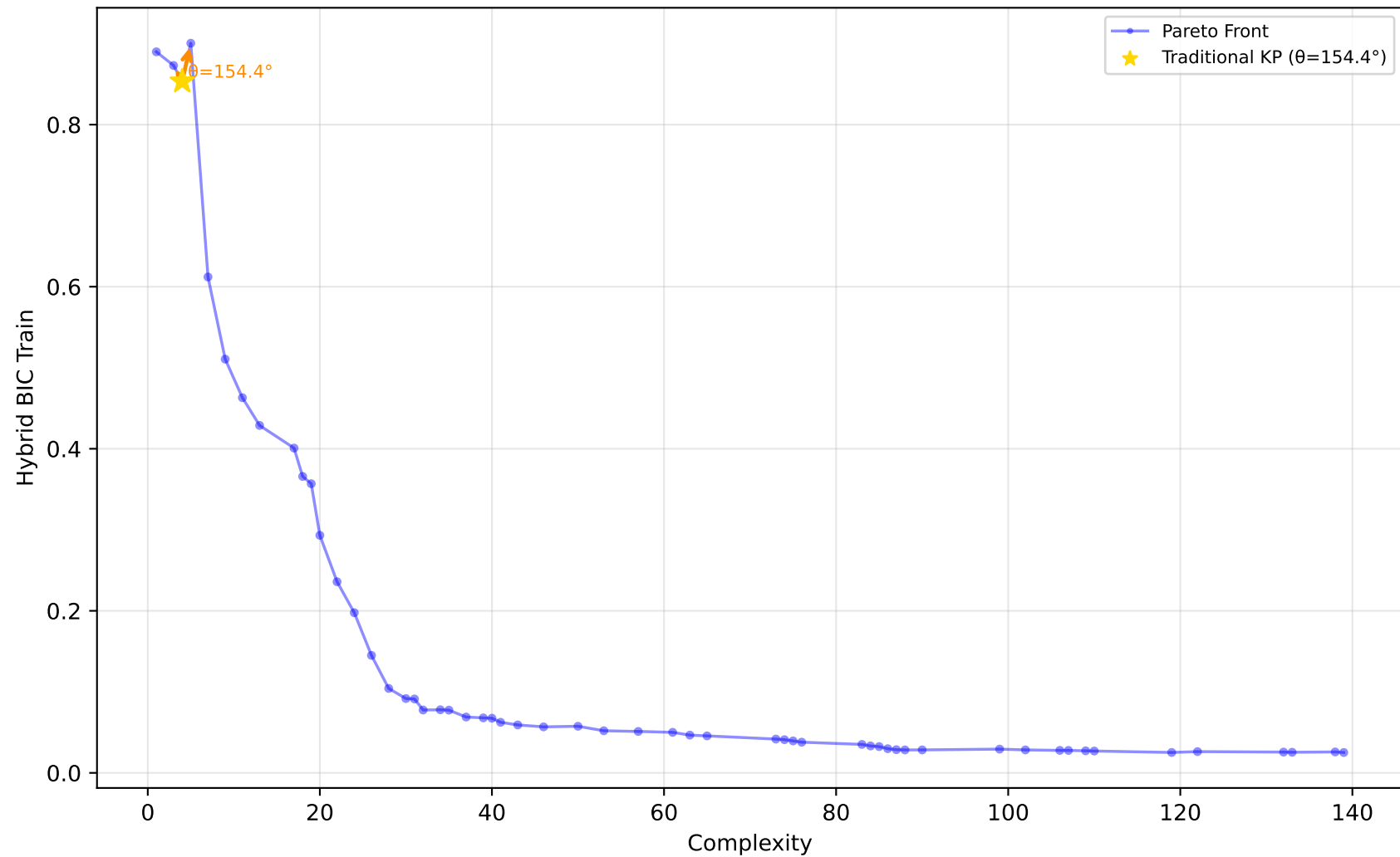
227_cpu_small - Run 3 - SVP - Hybrid BIC Train \lambda_1=0.00, \lambda_2=1.00, \lambda_3=0.00 | Difficulty: 1.00 | Method: hmr
