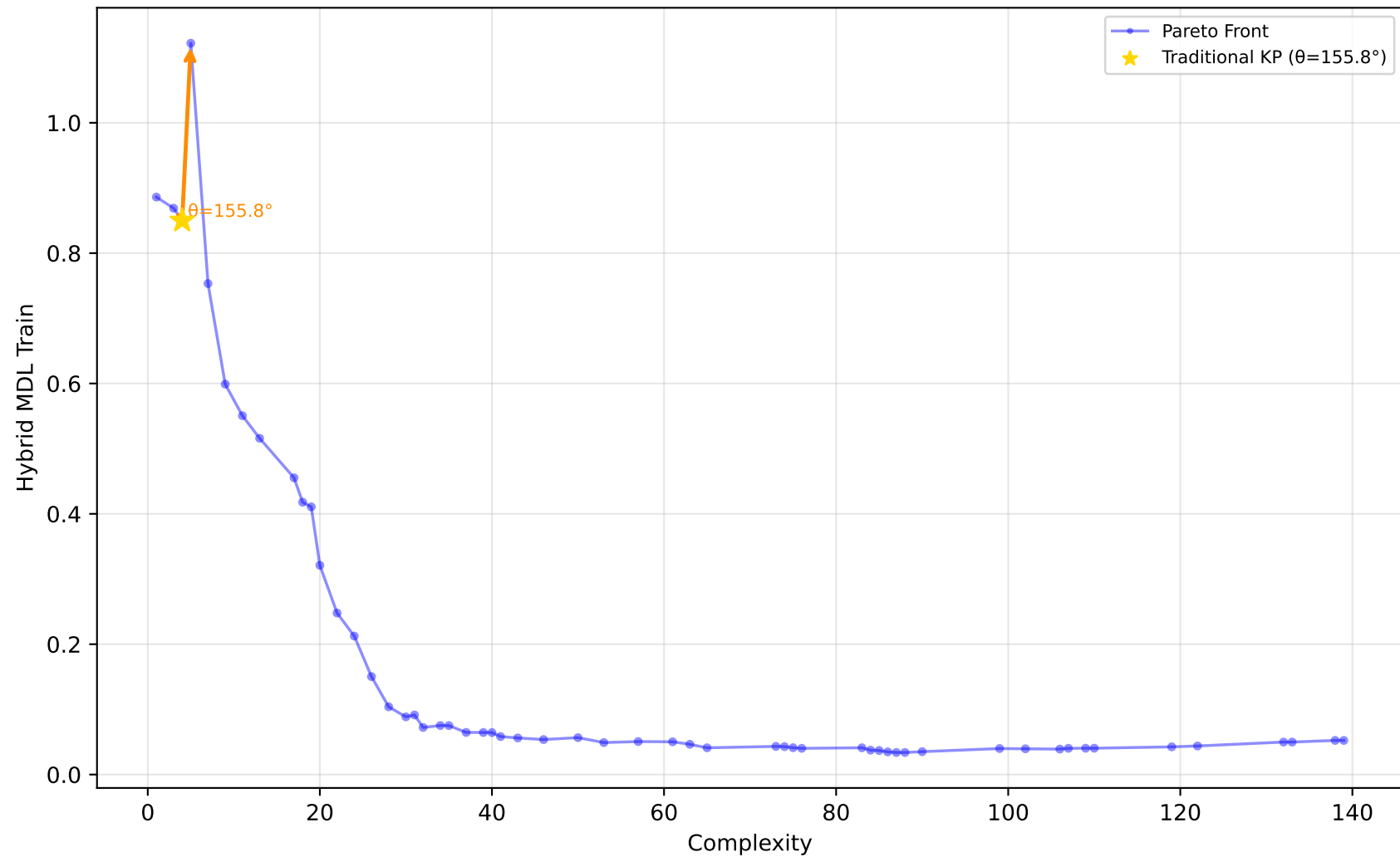
227_cpu_small - Run 3 - SVP - Hybrid MDL Train \lambda_1=0.00, \lambda_2=0.80, \lambda_3=0.30 | Difficulty: 1.00 | Method: hmr
