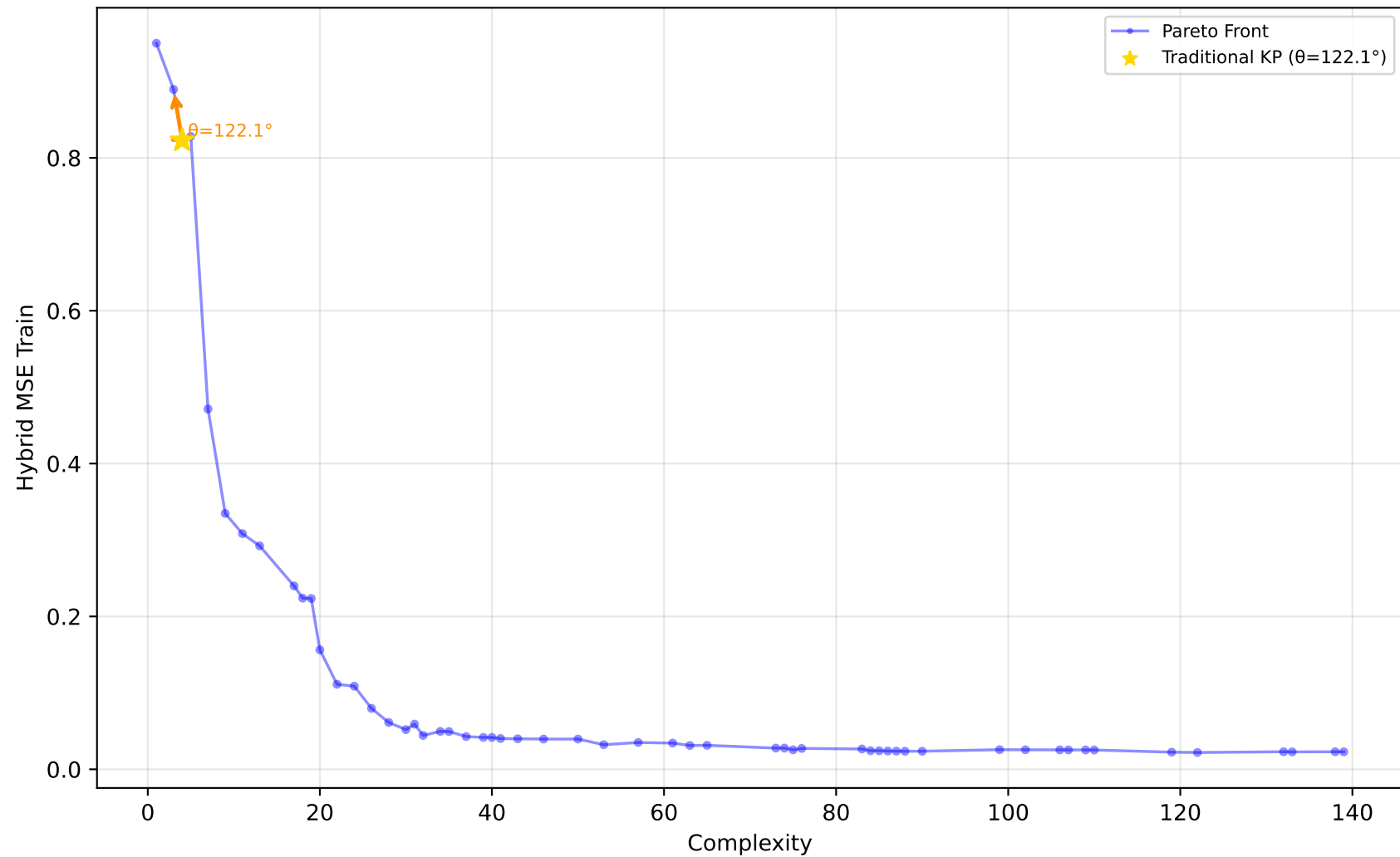
227_cpu_small - Run 3 - SVP - Hybrid MSE Train \lambda_1=0.00, \bar{\lambda}_2=0.80, \lambda_3=0.30 | Difficulty: 1.00 | Method: hmr
