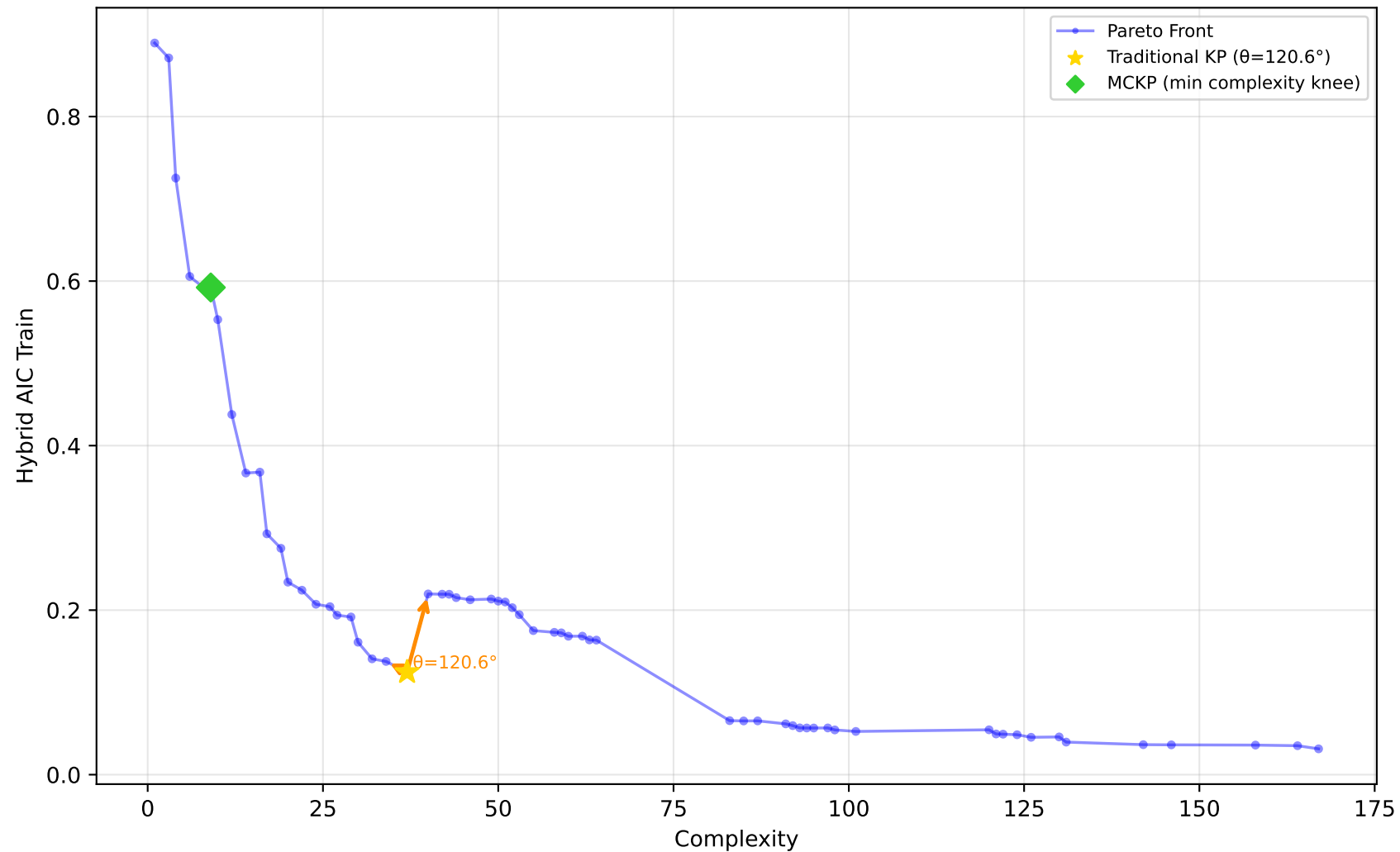
227_cpu_small - Run 4 - MVP - Hybrid AIC Train \lambda_1=0.00, \bar{\lambda}_2=0.90, \lambda_3=0.10 | Difficulty: 1.00 | Method: hmr
