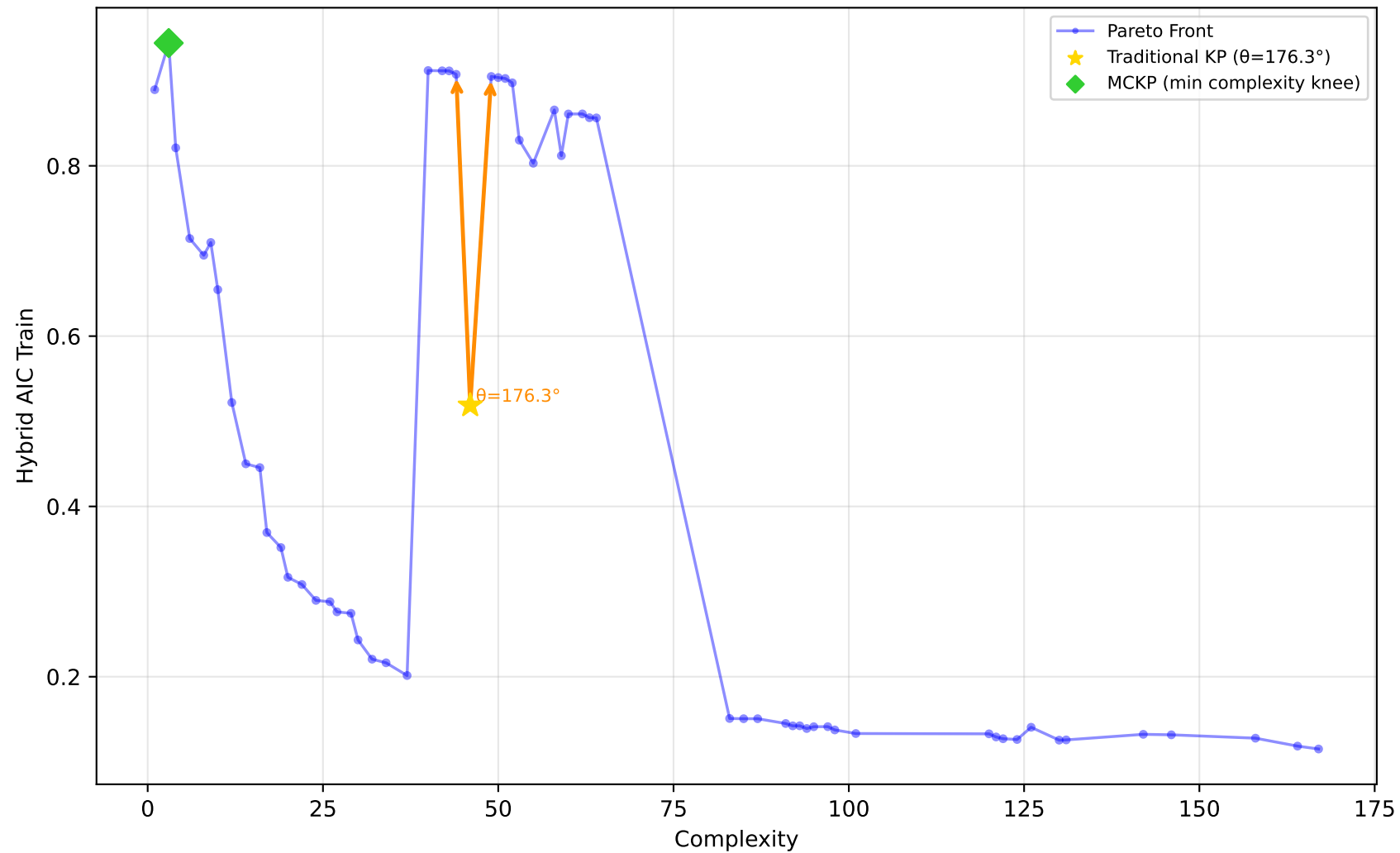
227_cpu_small - Run 4 - MVP - Hybrid AIC Train \lambda_1=0.80 , \lambda_2=0.20 , \lambda_3=0.00 | Difficulty: 1.00 | Method: hmr
