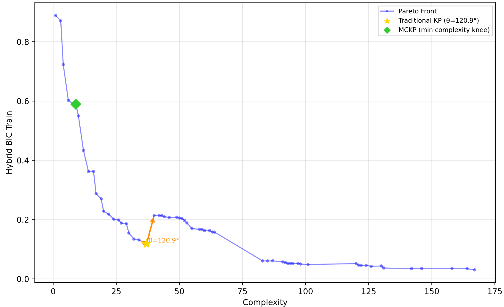
227_cpu_small - Run 4 - MVP - Hybrid BIC Train \lambda_1=0.00, \bar{\lambda}_2=0.90, \lambda_3=0.10 | Difficulty: 1.00 | Method: hmr
