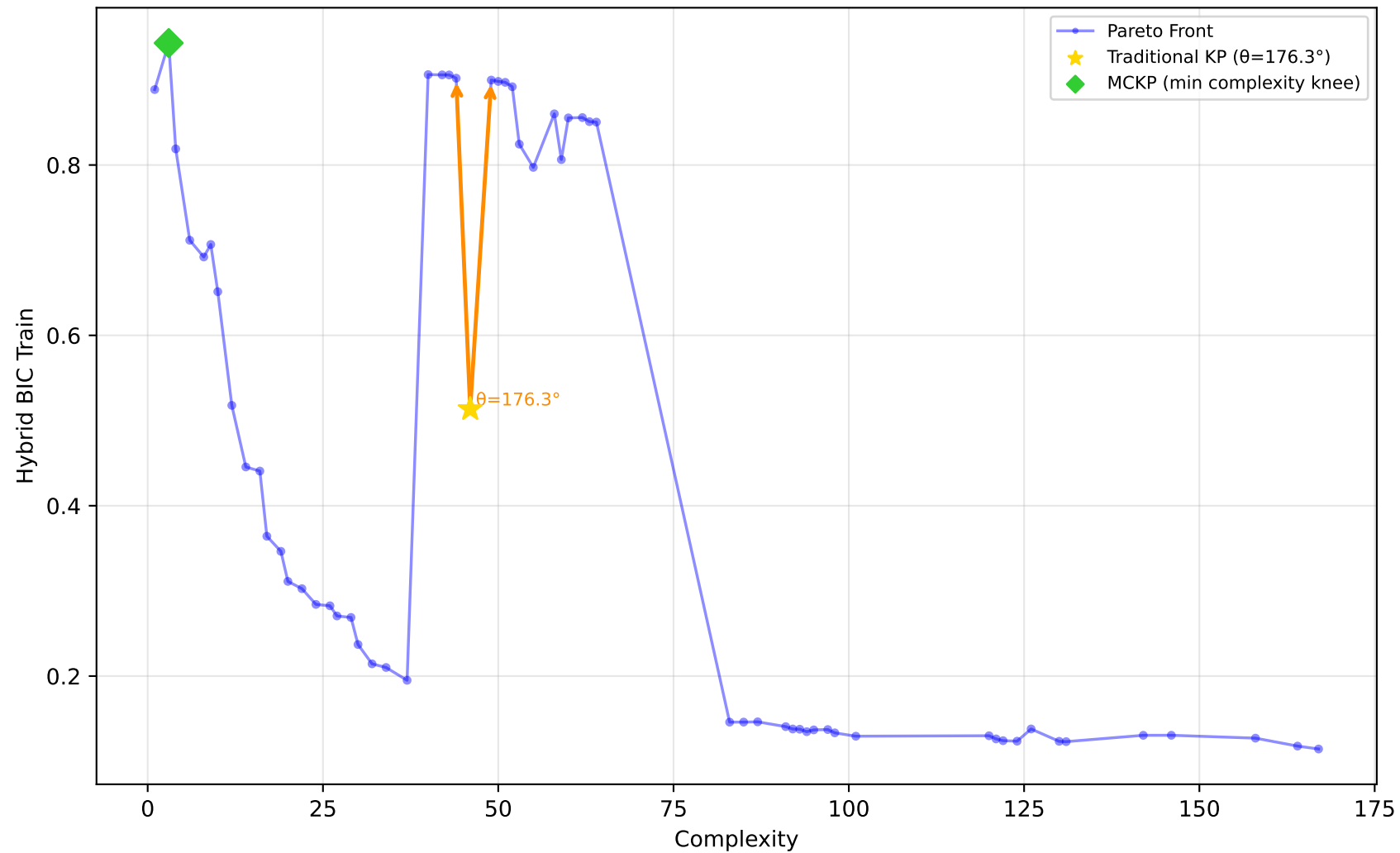
227_cpu_small - Run 4 - MVP - Hybrid BIC Train \lambda_1=0.80 , \lambda_2=0.20 , \lambda_3=0.00 | Difficulty: 1.00 | Method: hmr
