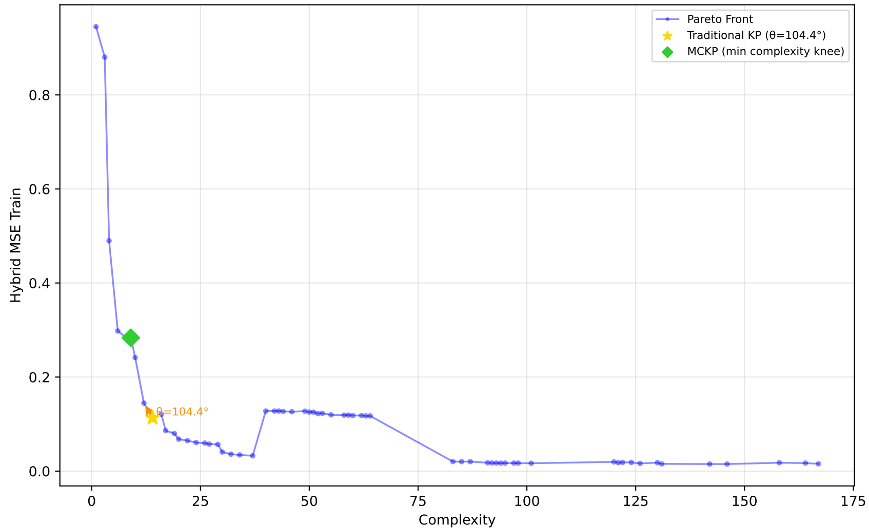
227_cpu_small - Run 4 - MVP - Hybrid MSE Train \lambda_1=0.00, \bar{\lambda}_2=0.90, \lambda_3=0.10 | Difficulty: 1.00 | Method: hmr
