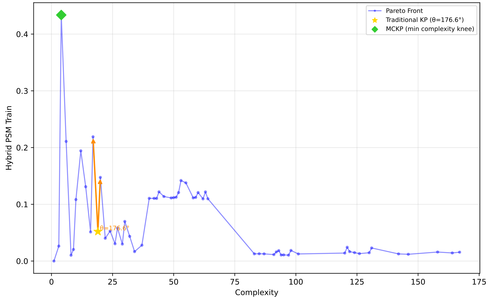
227_cpu_small - Run 4 - MVP - Hybrid PSM Train \lambda_1=0.00, \bar{\lambda}_2=0.90, \lambda_3=0.10 | Difficulty: 1.00 | Method: hmr
