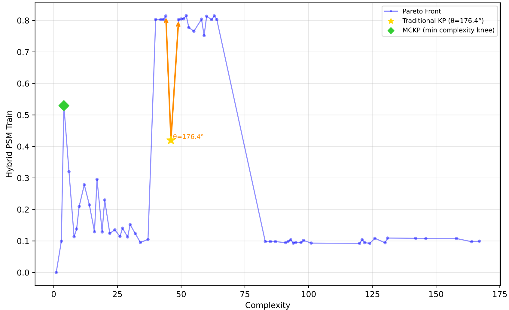
227_cpu_small - Run 4 - MVP - Hybrid PSM Train \lambda_1=0.80, \lambda_2=0.20, \lambda_3=0.00 | Difficulty: 1.00 | Method: hmr
