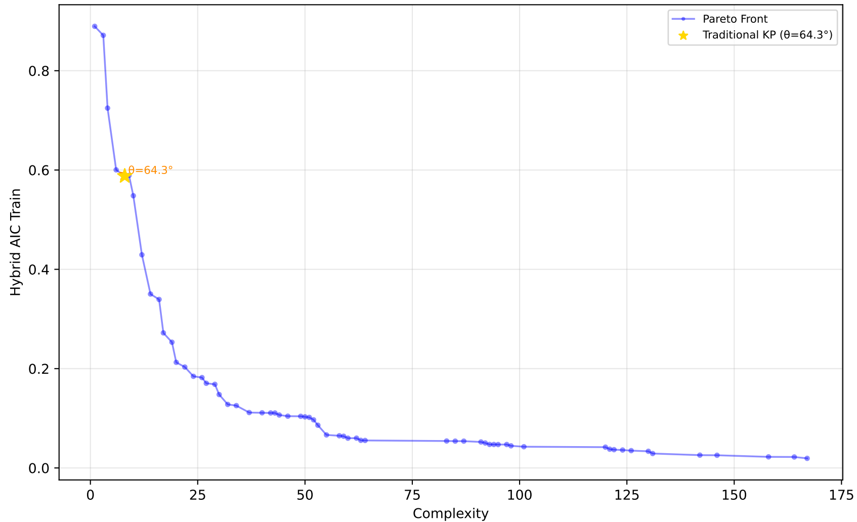
227_cpu_small - Run 4 - SVP - Hybrid AIC Train \lambda_1=0.00, \lambda_2=1.00, \lambda_3=0.00 | Difficulty: 1.00 | Method: hmr
