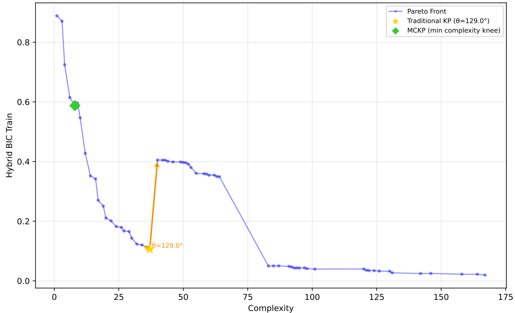
227_cpu_small - Run 4 - SVP - Hybrid BIC Train \lambda_1=0.00, \lambda_2=0.80, \lambda_3=0.30 | Difficulty: 1.00 | Method: hmr
