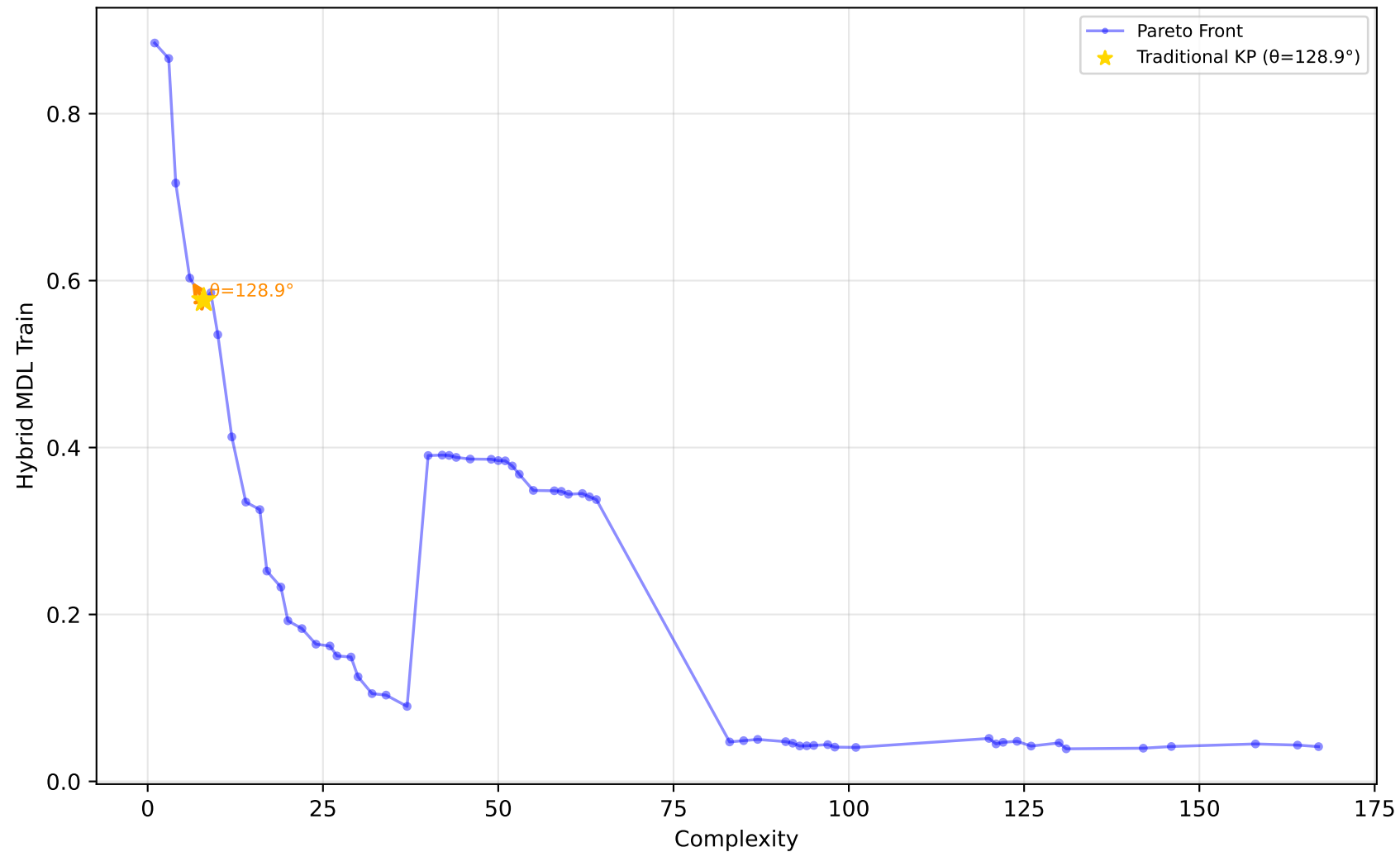
227_cpu_small - Run 4 - SVP - Hybrid MDL Train \lambda_1=0.00, \bar{\lambda}_2=0.80, \lambda_3=0.30 | Difficulty: 1.00 | Method: hmr
