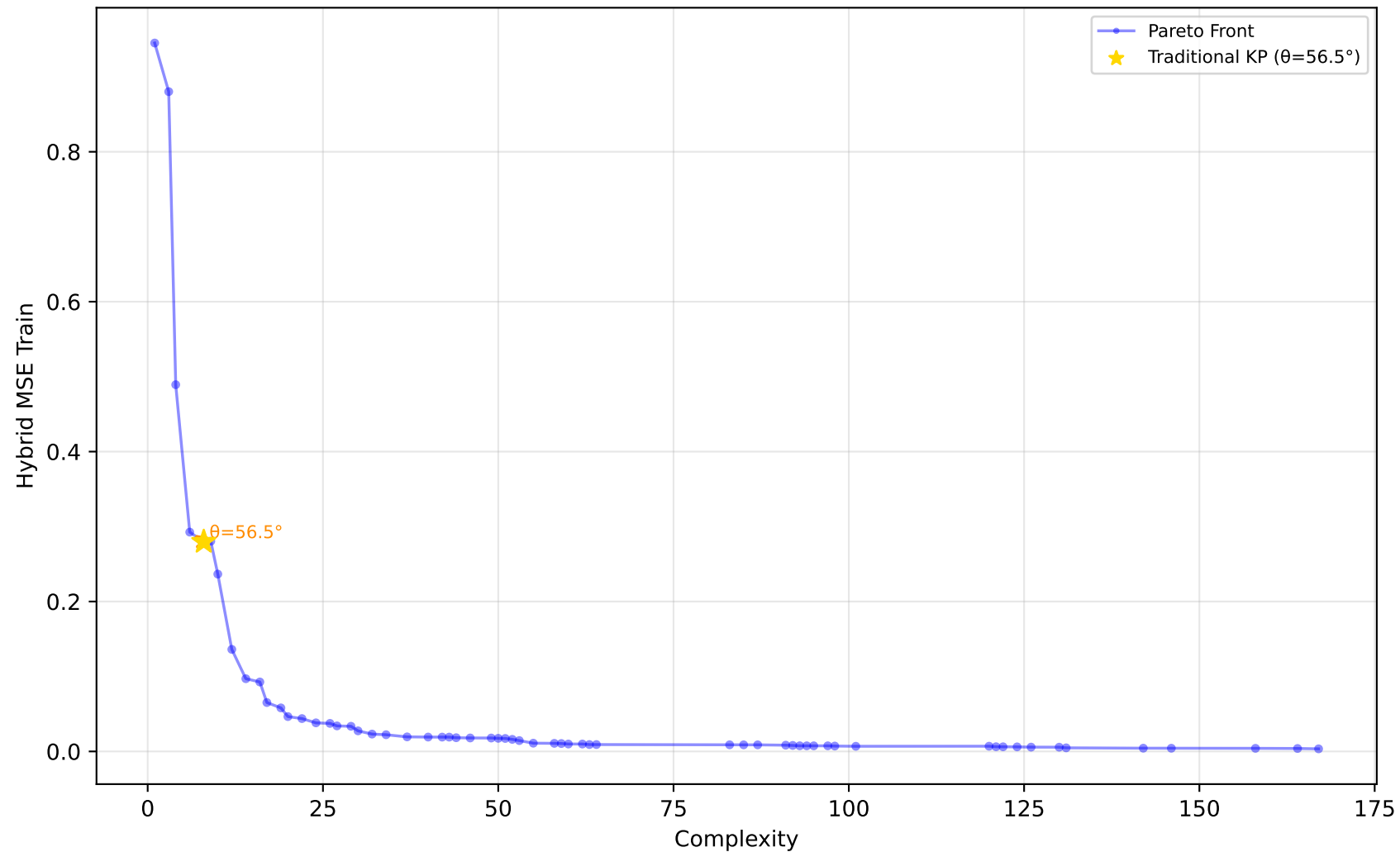
227_cpu_small - Run 4 - SVP - Hybrid MSE Train \lambda_1=0.00, \bar{\lambda}_2=1.00, \lambda_3=0.00 | Difficulty: 1.00 | Method: hmr
