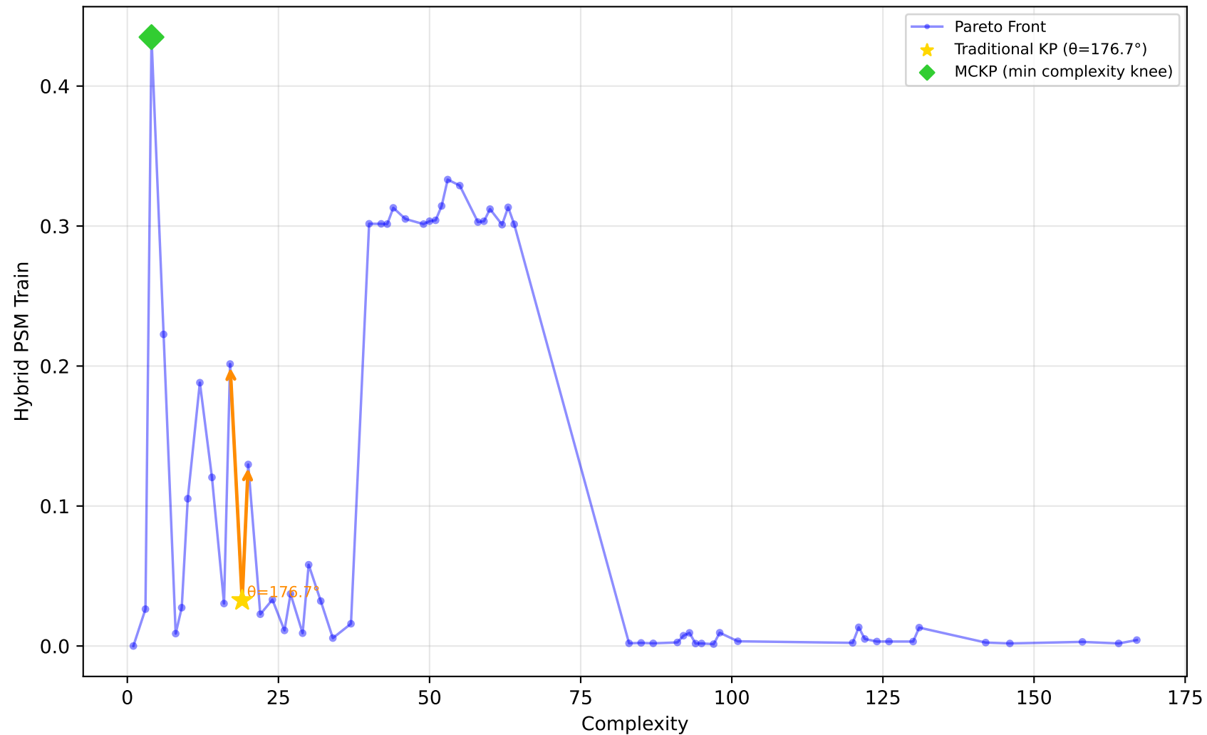
227_cpu_small - Run 4 - SVP - Hybrid PSM Train \lambda_1=0.00, \bar{\lambda}_2=0.80, \lambda_3=0.30 | Difficulty: 1.00 | Method: hmr
