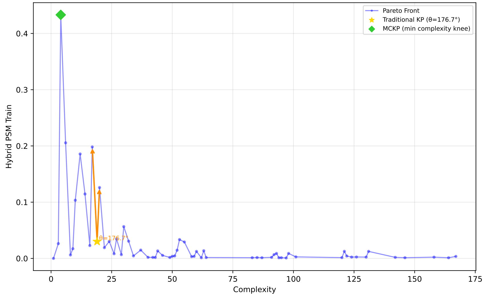
227_cpu_small - Run 4 - SVP - Hybrid PSM Train \lambda_1=0.00, \bar{\lambda}_2=1.00, \lambda_3=0.00 | Difficulty: 1.00 | Method: hmr
