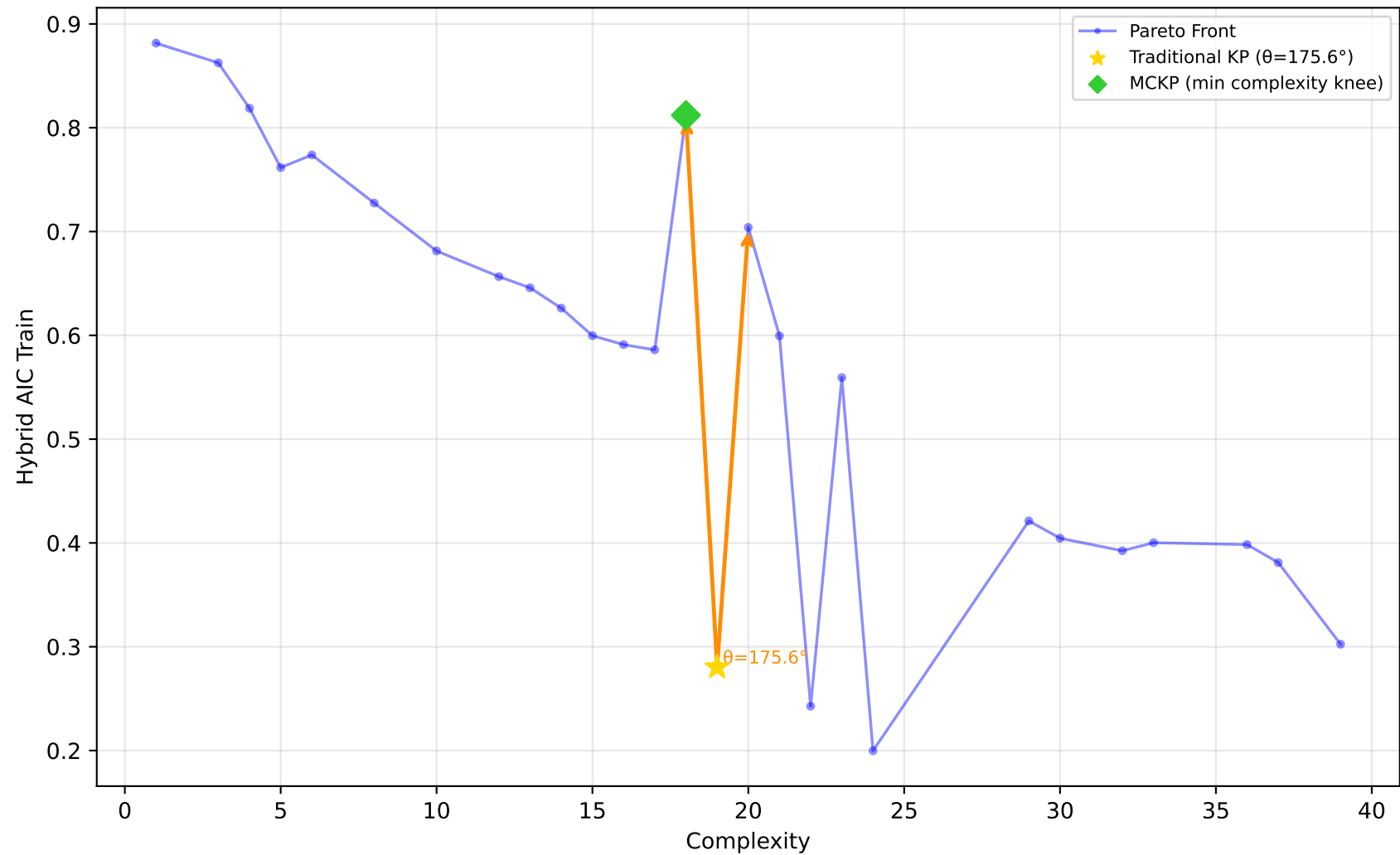
227_cpu_small - Run 5 - MVP - Hybrid AIC Train \lambda_1=0.00, \bar{\lambda}_2=0.90, \lambda_3=0.10 | Difficulty: 1.00 | Method: hmr
