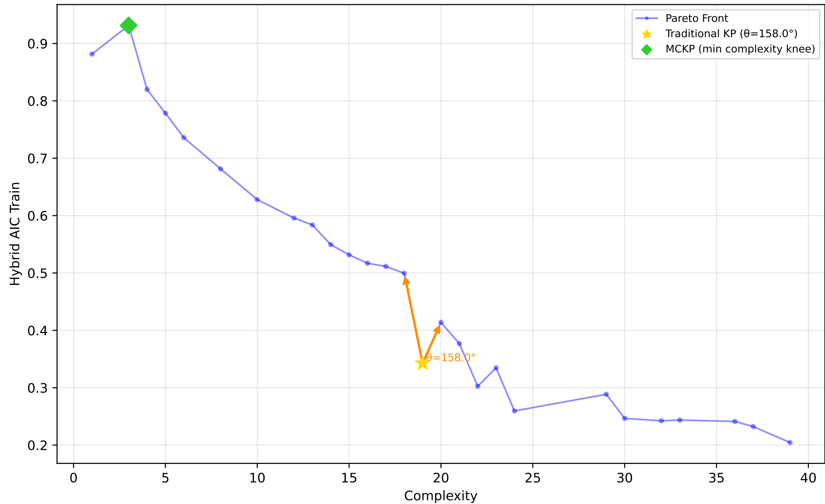
227_cpu_small - Run 5 - MVP - Hybrid AIC Train \lambda_1=0.80, \bar{\lambda}_2=0.20, \lambda_3=0.00 | Difficulty: 1.00 | Method: hmr
