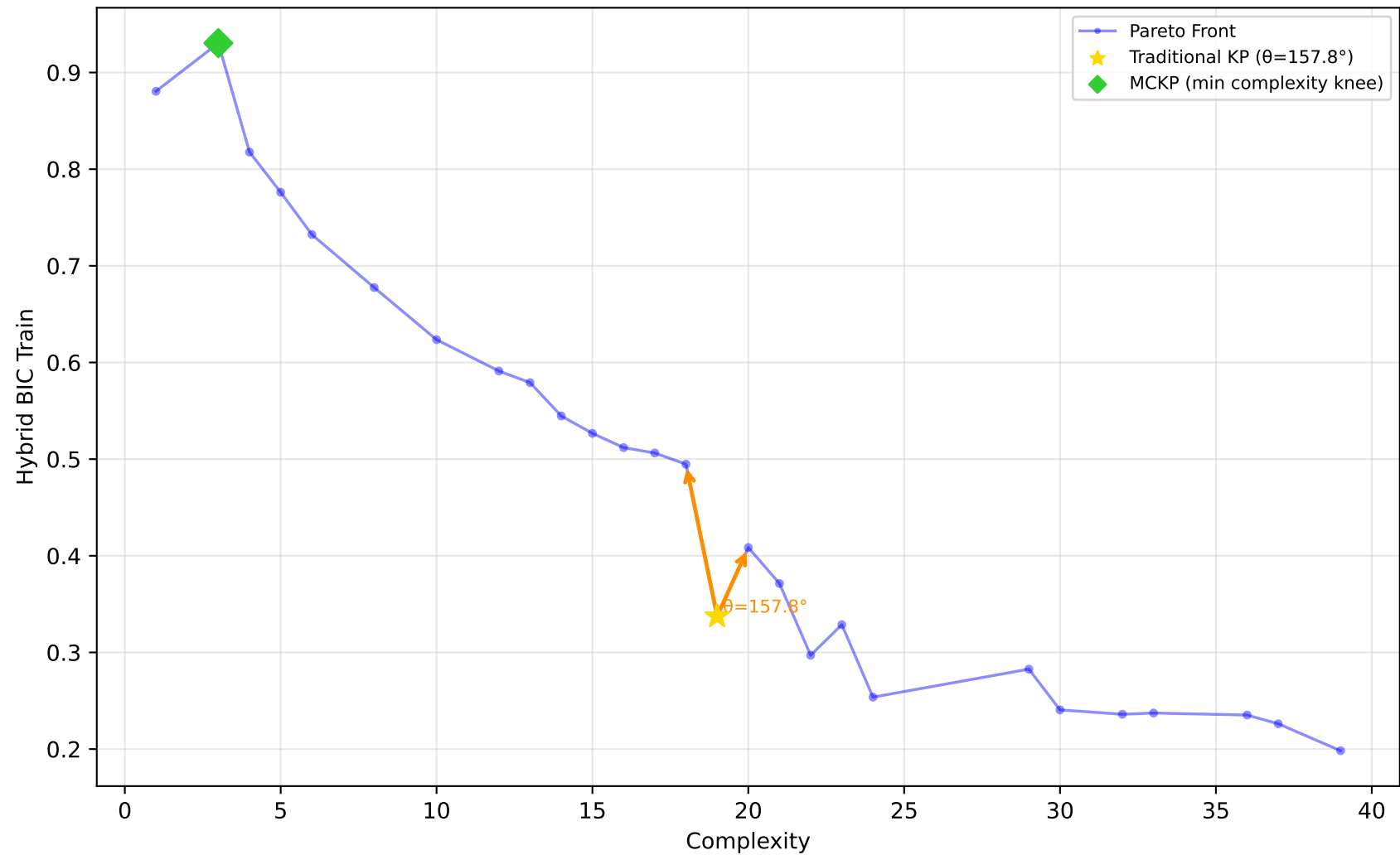
227_cpu_small - Run 5 - MVP - Hybrid BIC Train \lambda_1=0.80, \bar{\lambda}_2=0.20, \lambda_3=0.00 | Difficulty: 1.00 | Method: hmr
