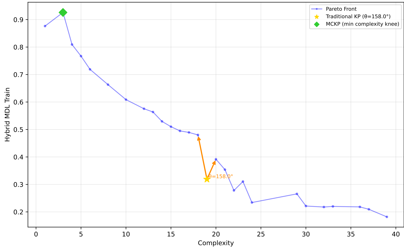
227_cpu_small - Run 5 - MVP - Hybrid MDL Train \lambda_1=0.80, \bar{\lambda}_2=0.20, \lambda_3=0.00 | Difficulty: 1.00 | Method: hmr
