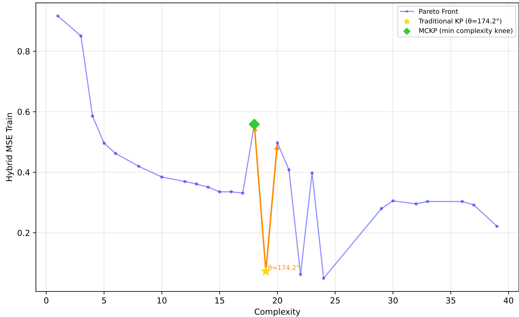
227_cpu_small - Run 5 - MVP - Hybrid MSE Train \lambda_1=0.00, \lambda_2=0.90, \lambda_3=0.10 | Difficulty: 1.00 | Method: hmr
