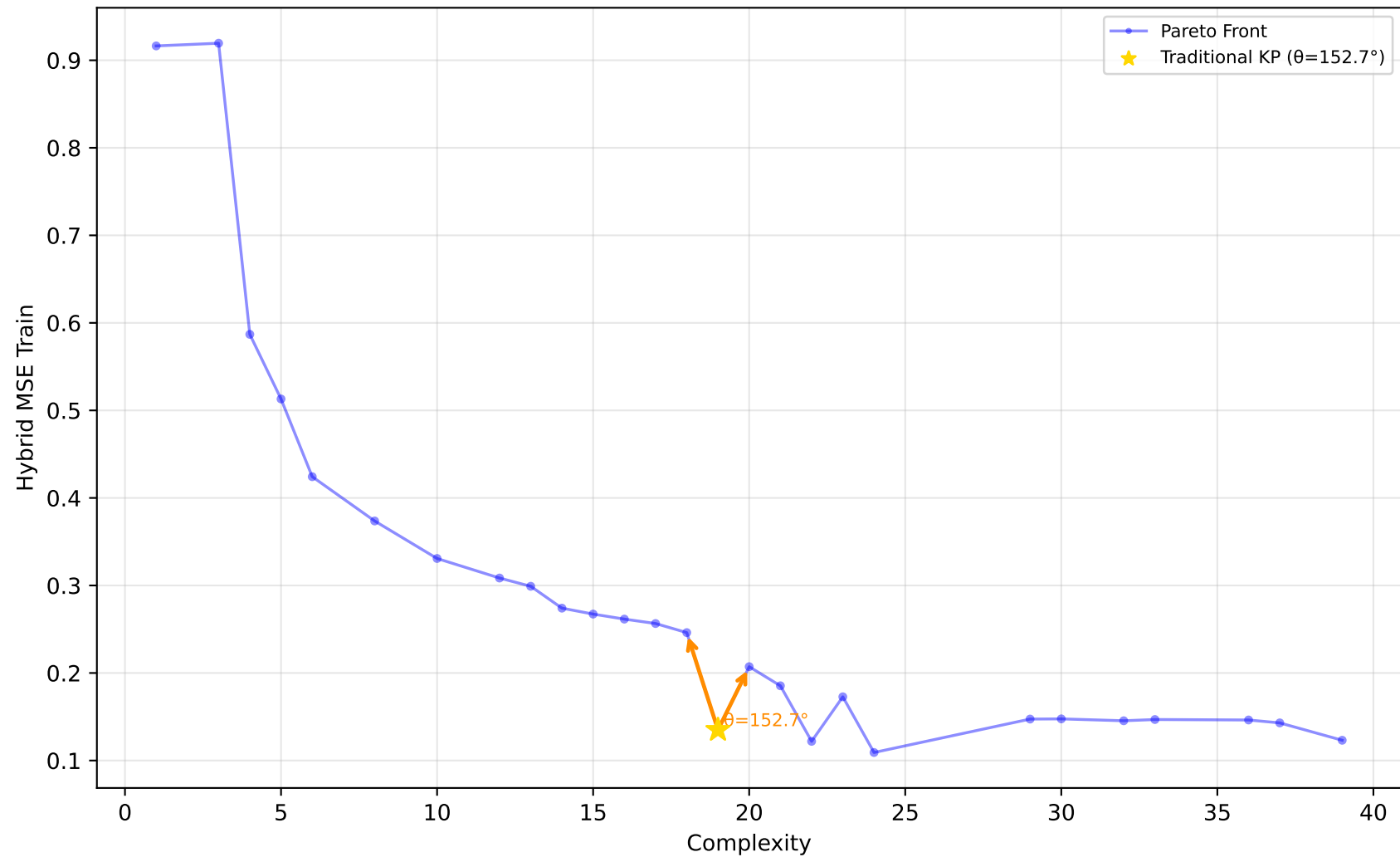
227_cpu_small - Run 5 - MVP - Hybrid MSE Train \lambda_1=0.80, \bar{\lambda}_2=0.20, \lambda_3=0.00 | Difficulty: 1.00 | Method: hmr
