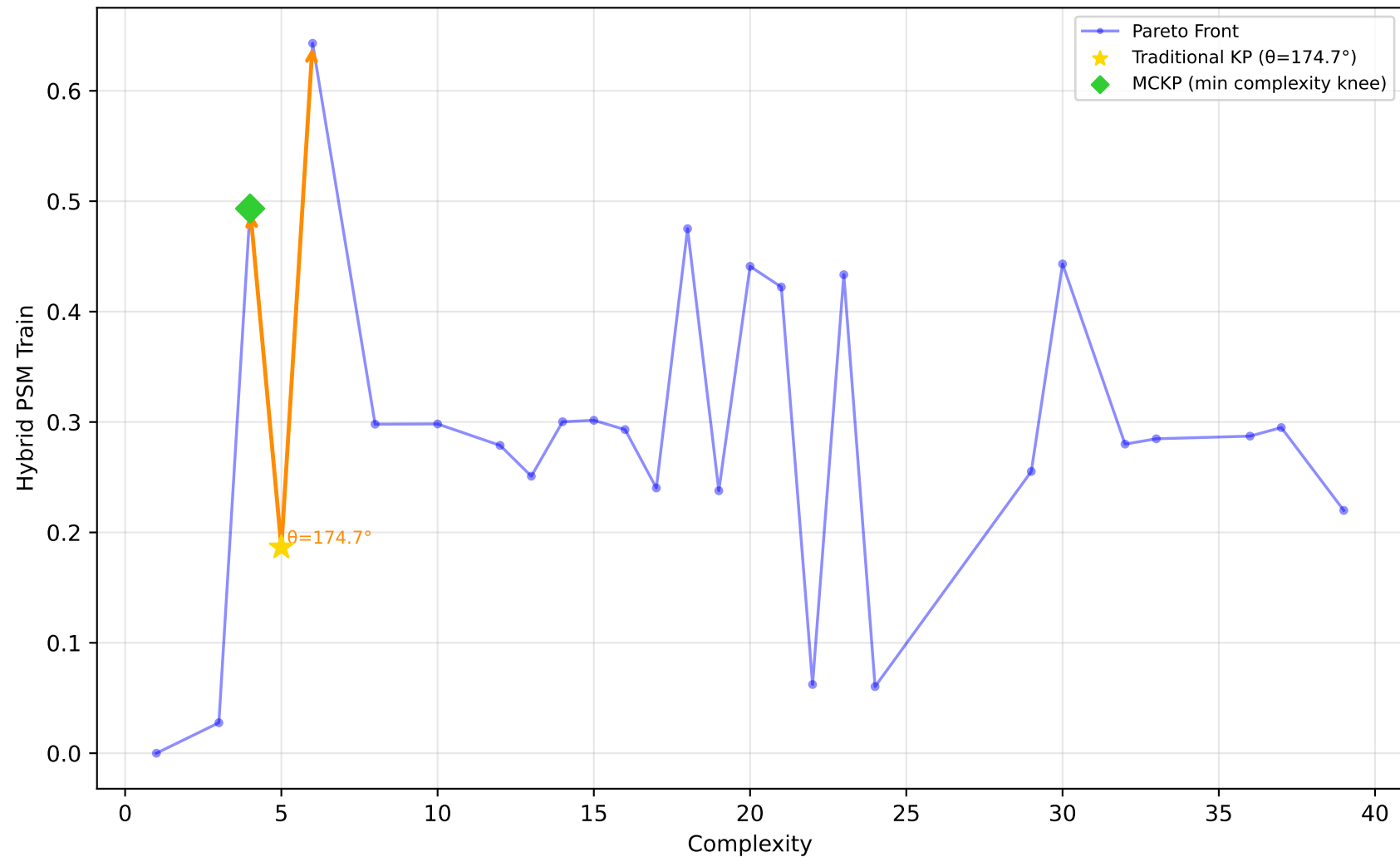
227_cpu_small - Run 5 - MVP - Hybrid PSM Train \lambda_1=0.00, \bar{\lambda}_2=0.90, \lambda_3=0.10 | Difficulty: 1.00 | Method: hmr
