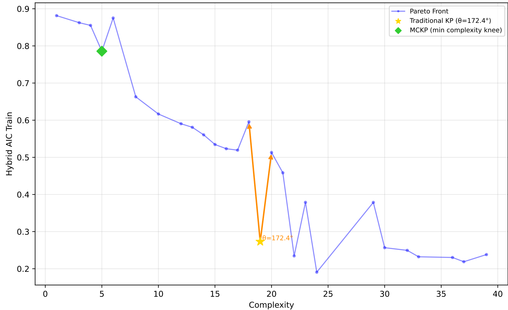
227_cpu_small - Run 5 - SVP - Hybrid AIC Train \lambda_1=0.00, \bar{\lambda}_2=0.80, \lambda_3=0.30 | Difficulty: 1.00 | Method: hmr
