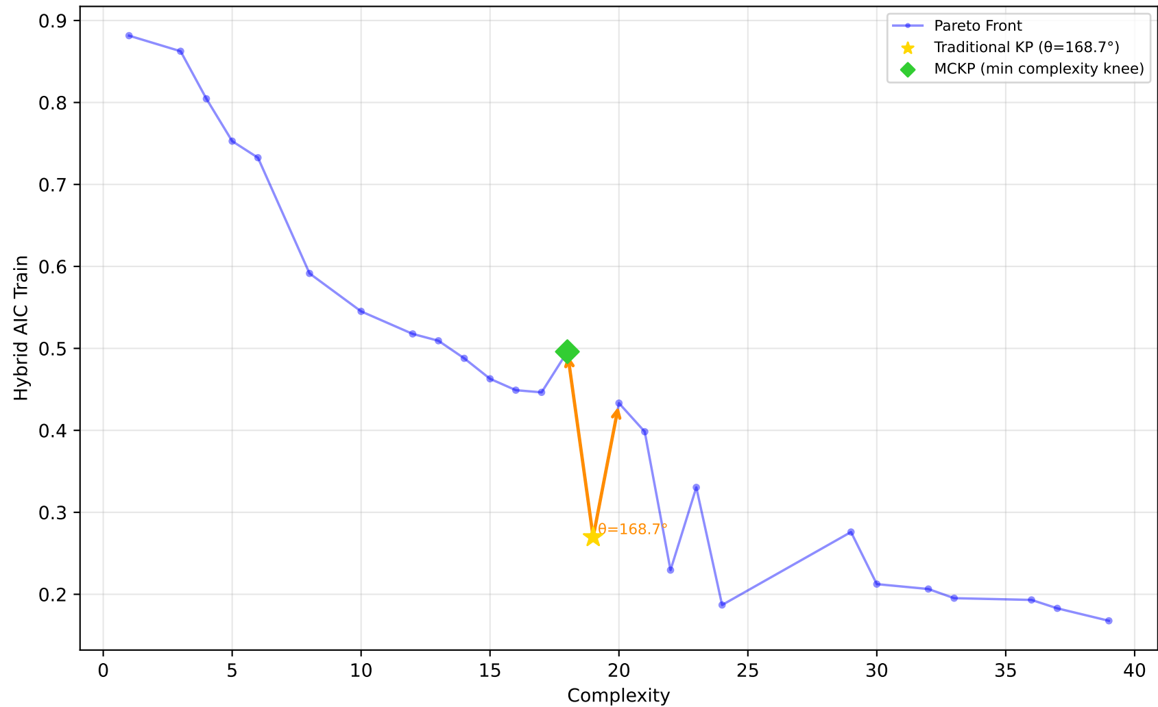
227_cpu_small - Run 5 - SVP - Hybrid AIC Train \lambda_1=0.00, \lambda_2=1.00, \lambda_3=0.00 | Difficulty: 1.00 | Method: hmr
