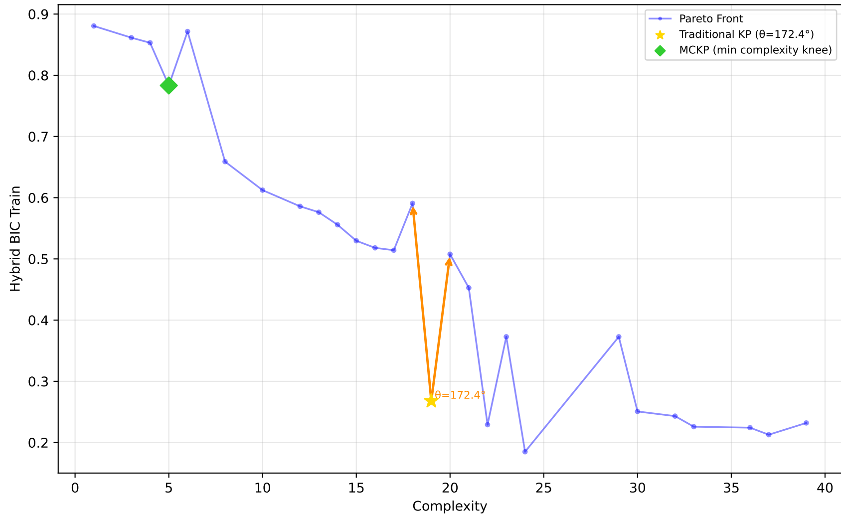
227_cpu_small - Run 5 - SVP - Hybrid BIC Train \lambda_1=0.00, \bar{\lambda}_2=0.80, \lambda_3=0.30 | Difficulty: 1.00 | Method: hmr
