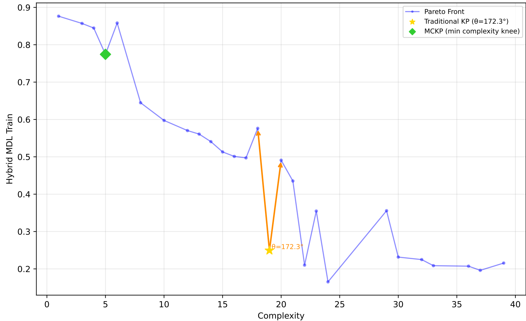
227_cpu_small - Run 5 - SVP - Hybrid MDL Train \lambda_1=0.00, \bar{\lambda}_2=0.80, \lambda_3=0.30 | Difficulty: 1.00 | Method: hmr
