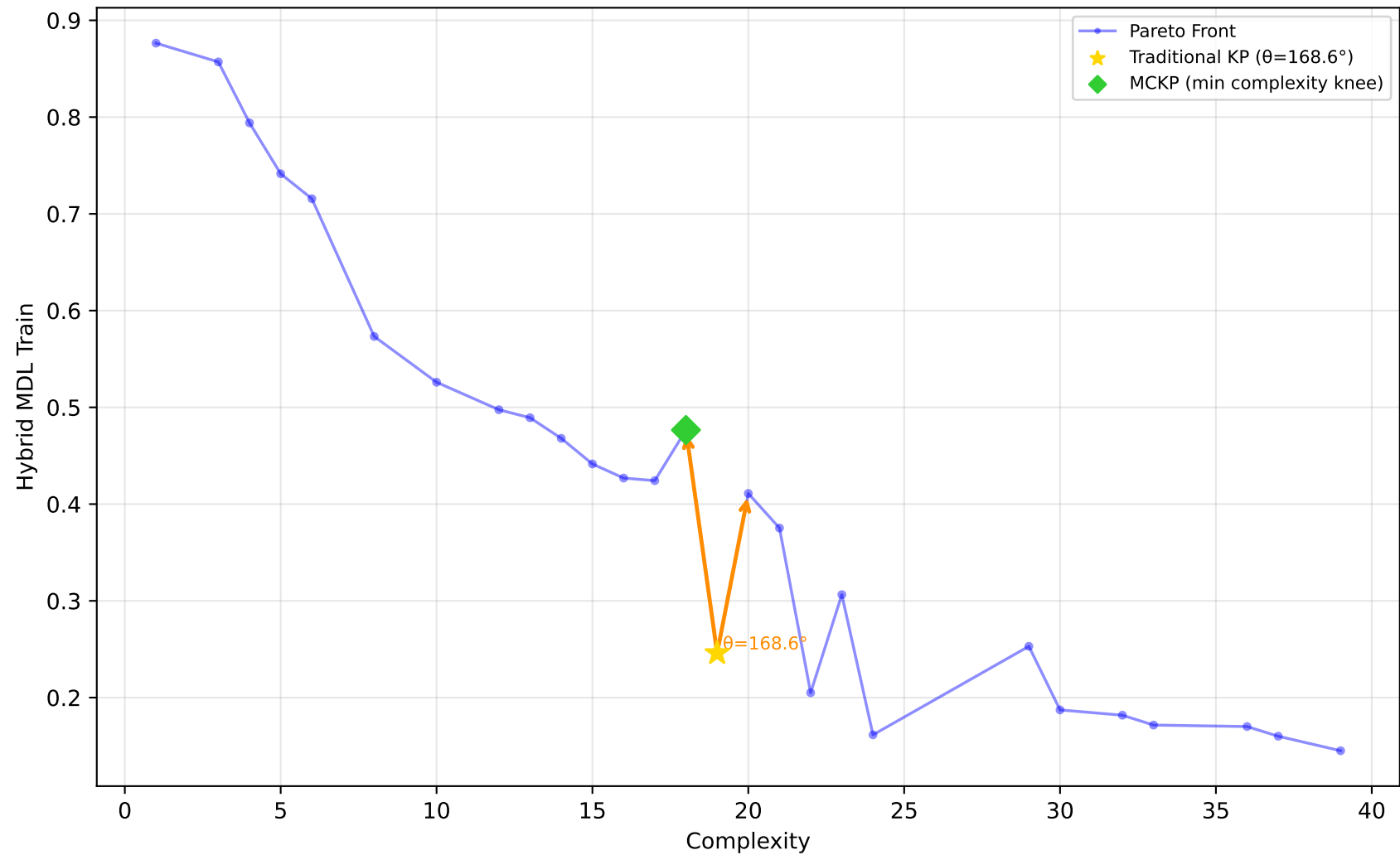
227_cpu_small - Run 5 - SVP - Hybrid MDL Train \lambda_1=0.00, \bar{\lambda}_2=1.00, \lambda_3=0.00 | Difficulty: 1.00 | Method: hmr
