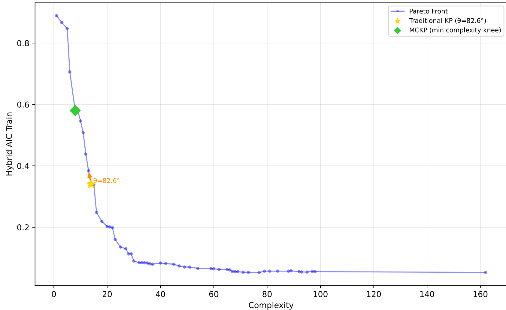
227_cpu_small - Run 6 - MVP - Hybrid AIC Train \lambda_1=0.00, \bar{\lambda}_2=0.90, \lambda_3=0.10 | Difficulty: 1.00 | Method: hmr
