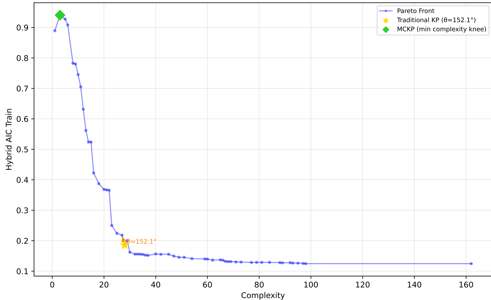
227_cpu_small - Run 6 - MVP - Hybrid AIC Train \lambda_1=0.80, \bar{\lambda}_2=0.20, \lambda_3=0.00 | Difficulty: 1.00 | Method: hmr
