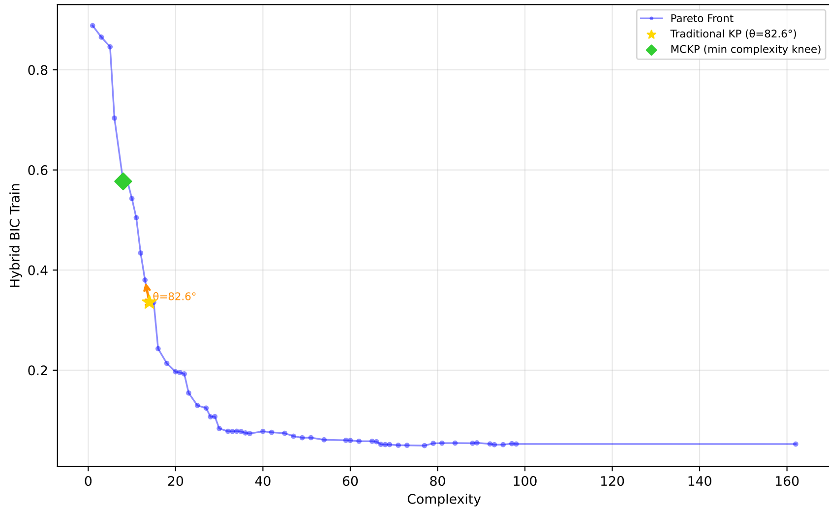
227_cpu_small - Run 6 - MVP - Hybrid BIC Train \lambda_1=0.00, \bar{\lambda}_2=0.90, \lambda_3=0.10 | Difficulty: 1.00 | Method: hmr
